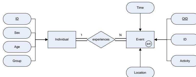
Figure 4: Data Model
