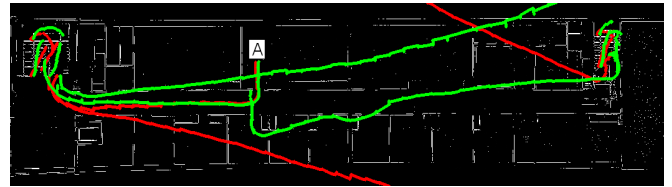
Fig. 3. Trajectories of two foot-mounted IMUs. Coordinates and heading from the emergency map are used as measurement for the EKF.
