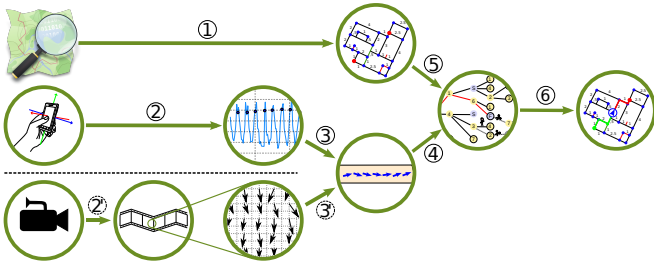
Fig. 4. Flow of information during navigation using FootPath [10]. (1) The application obtains map material, e.g., from the photograph of an evacuation plan. (2) Using the inbuilt accelerometer, a mobile phone detects steps. (3) The detected steps are combined with heading information using the inbuilt magnetometer. Alternatively, (2') the smartphone camera records and compresses a video of the floor. Our system reads out the motion vectors. (3') The detected motion vectors are transformed into virtual steps together with heading information from the magnetometer. (4) The detected steps are mapped onto a map. (5) The base map provides the available orientations and candidate paths. (6) The user gets feedback about the current most probable position, based on the detected scores.
