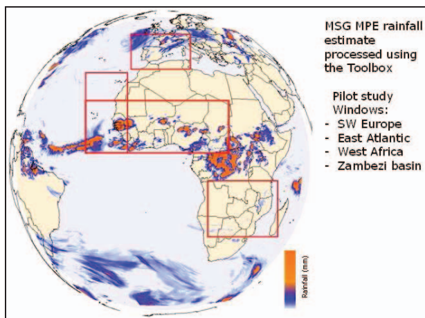
Figure 5: MSG Meteosat-9 precipitation estimate
