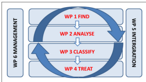
Figure 3 Project structure [6]
