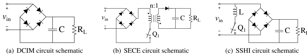
Figure 1 : Previous circuits
