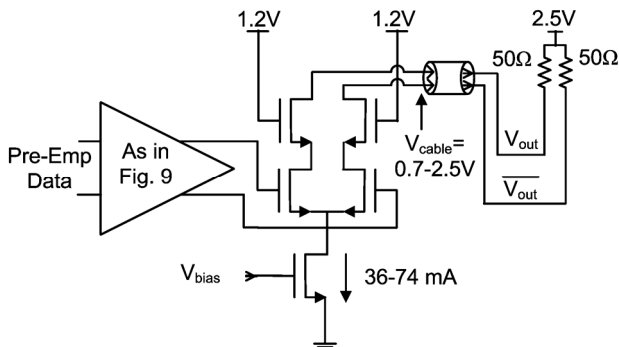
Fig. 13. Line driver of chip 2 with cable and termination.
