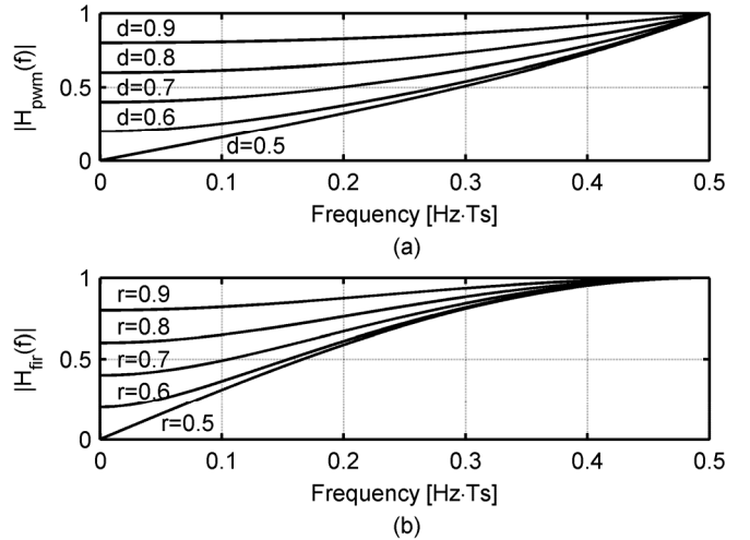
Fig. 5. Calculated normalized magnitude of filter transfer. (a). PWM-PE filter. (b). 2-tap SSF-PE filter.
