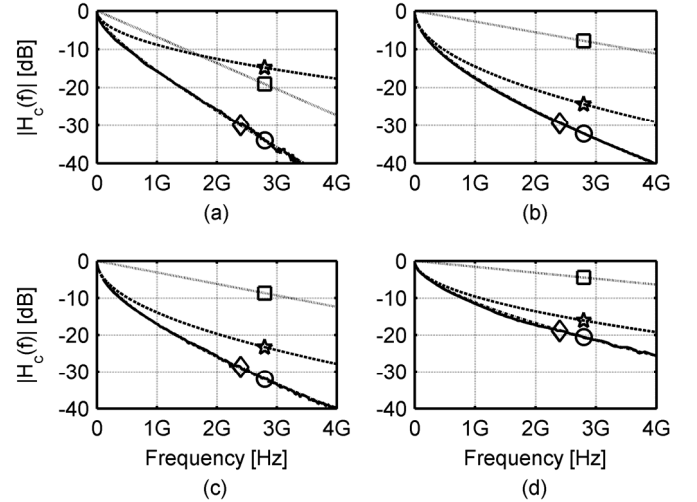
Fig. 6. Measured and modeled cable transfer functions. Diamond: measured S_{21} . Star: skin loss, model. Square: dielectric loss, model. Circle: total loss, model. (a). 25 m RG-58CU. (b). 130 m Aircom+. (c). 80 m Aircell7. (d). 15 m 10GBASE-CX4 24AWG. (Measured: S_{dd21} .)
