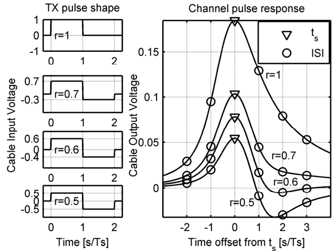
Fig. 4. TX pulse shapes ( T_s=200 ps) of SSF-PE filter with varying r parameter and simulated responses of 25 m RG-58CU cable.
