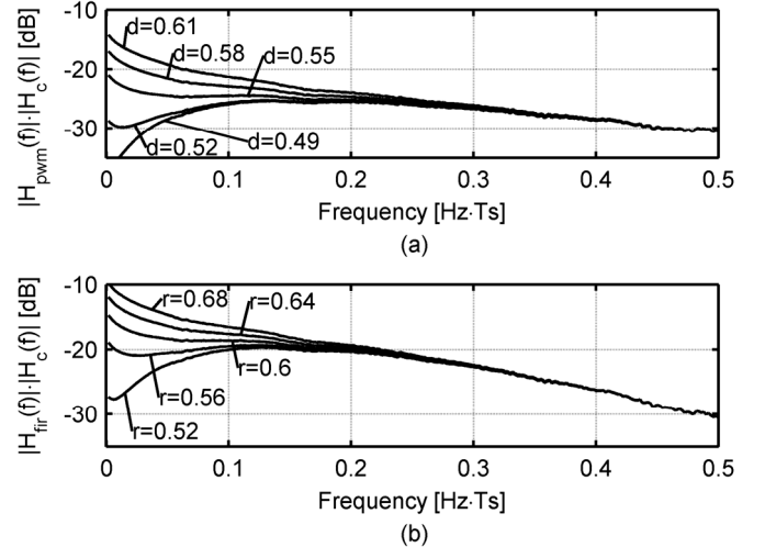
Fig. 7. Equalized transfer of 25 m RG-58CU. (a). PWM. (b). 2-tap SSF.
