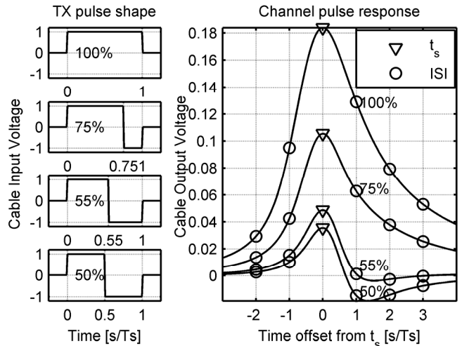
Fig. 3. TX pulse shapes ( T_s=200 ps) of PWM-PE filter with varying duty-cycles and simulated responses of 25 m RG-58CU cable.
