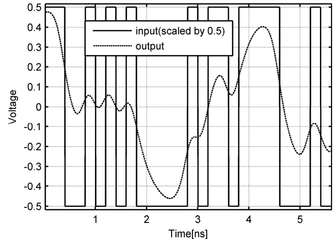
Fig. 1. Simulated response of 25 m RG-58CU coaxial cable to 5 Gb/s data.
