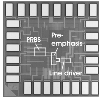
Fig 10. Microphotograph of chip 1, 1x1 mm 2 .
