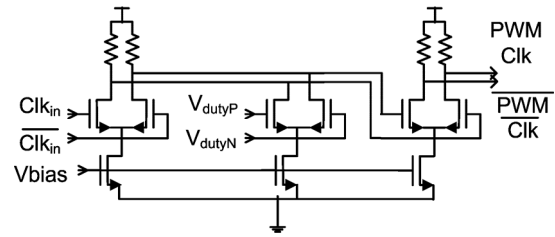
Fig. 14. Duty-cycle tuning circuit of chip 2.
