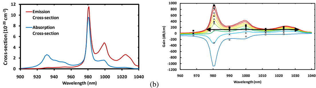
Fig. 2. Spectral information on \text{KGd}_{0.447}\text{Lu}_{0.078}\text{Yb}_{0.475}(\text{WO}_4)_2 : (a) Emission and absorption cross-sections, derived as the weighted average of spectroscopic data from the compounds \text{KGd}(\text{WO}_4)_2:\text{Yb}^{3+} , \text{KLu}(\text{WO}_4)_2:\text{Yb}^{3+} , and \text{KYb}(\text{WO}_4)_2 [17,18,9]. (b) Waveguide modal gain for different launched pump powers, calculated (lines) from the absorption and emission cross-sections presented in part (a) and measured (symbols); indication (arrow) of the spectral range with g_{\text{mod}} > 150 \text{ dB/cm} .
