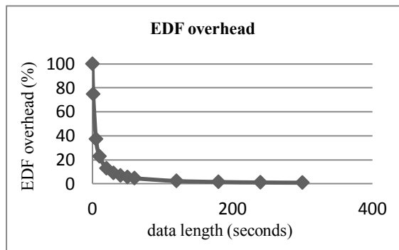
Figure 3: EDF overhead for the complete INTERACTION sensing system.
