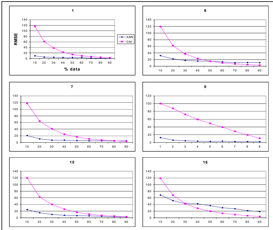
Figure 6: Model performances
