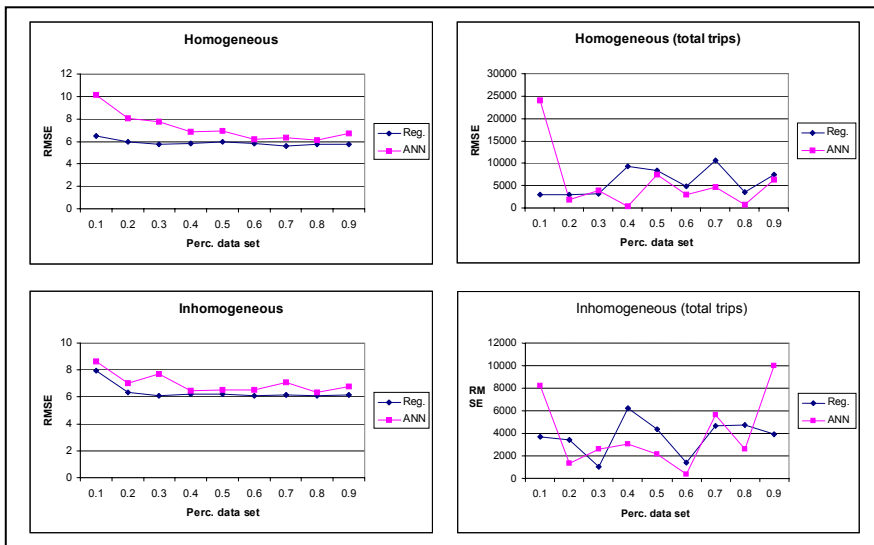
Figure 2: Performance of both methods in complexity cases 1 and 2 with scarce data.
