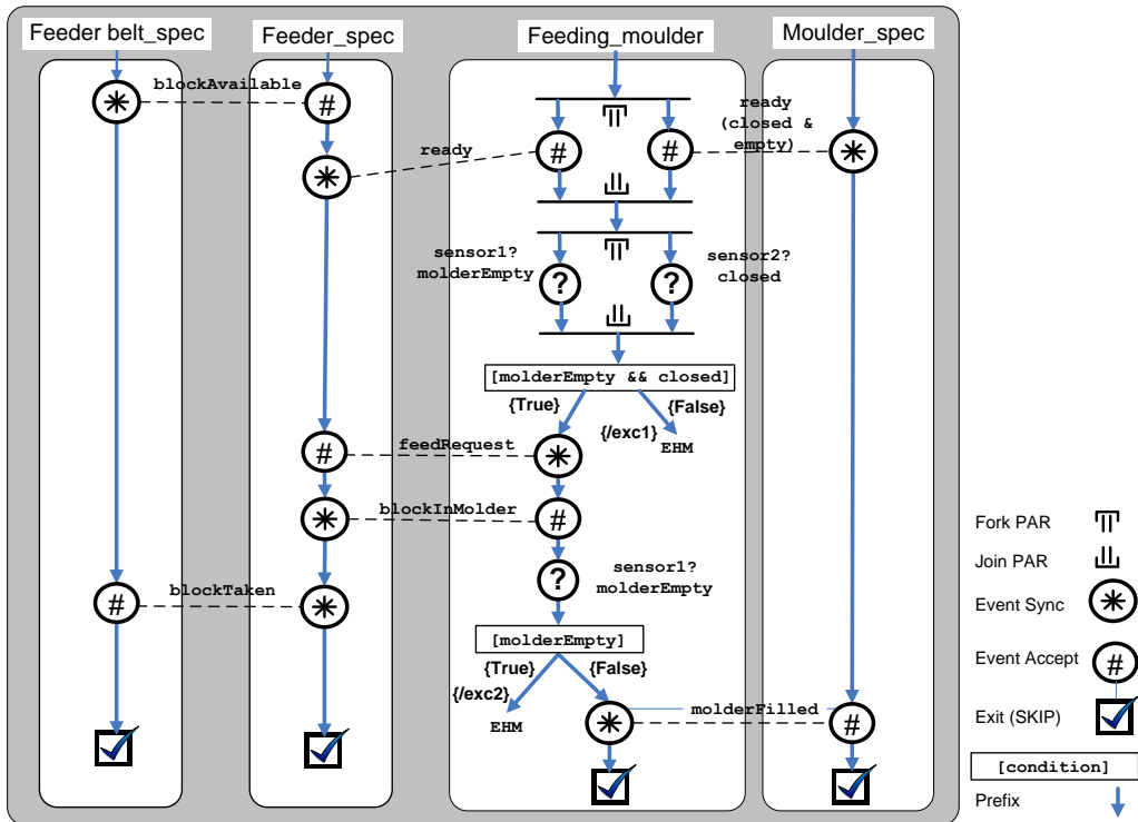
Figure 7. SystemCSP interaction contract between feederbelt, feeder and moulder (adapted from [8])
