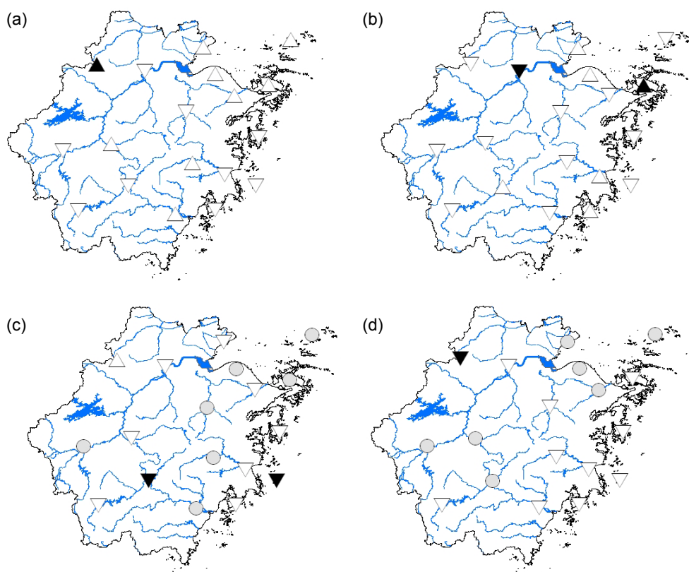
Fig. 1 (a) Precipitation trend in plum season; (b) trend of the number of precipitation days in plum season; (c) precipitation trend in typhoon season; (d) trend of the number of precipitation days in typhoon season. Here ○ represents no trend; Δ and ▲ represent positive and significant positive trends, respectively; ▽ and ▼ represent negative and significant negative trends, respectively.
