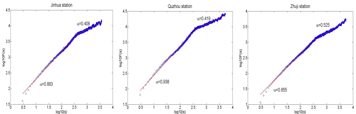
Fig. 2 Log–log plots of F(s) versus s of Jinhua station, Quzhou station and Zhuji station.
