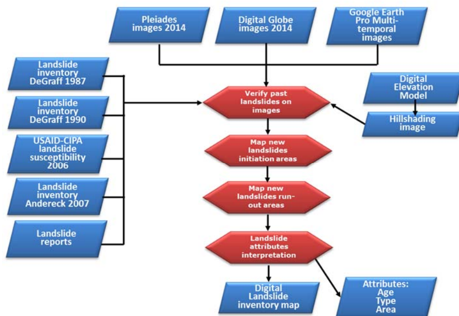
Figure 4-3: Method used for the generation of a landslide inventory map for Dominica
