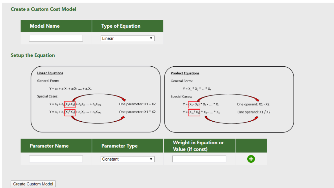
Fig. 5. Create a Custom Model.
