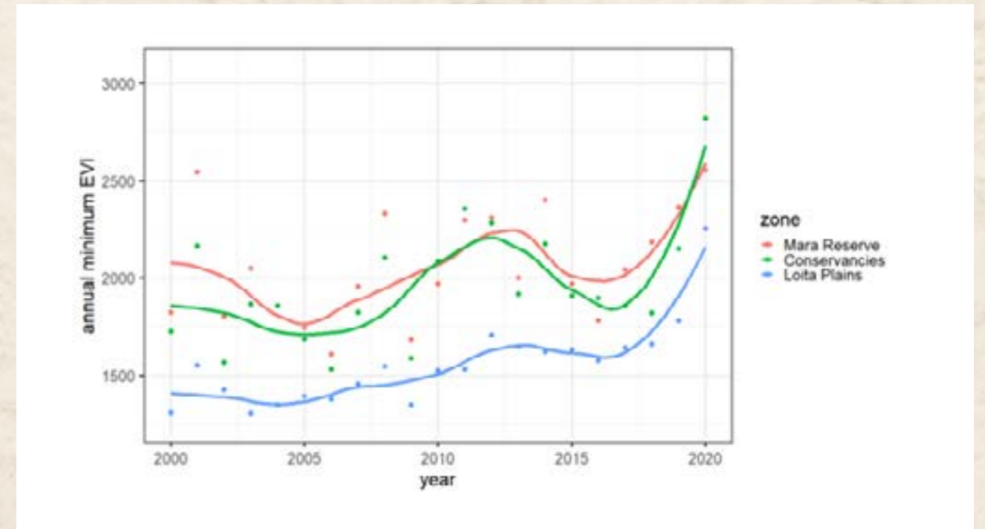
Fig 40. Trends in the minimum annual Enhanced Vegetation Index (EVI, and extended NDVI index measuring greenness of vegetation), calculated using 16-day MODIS composites, and spatially averaged over the three study area zones.
