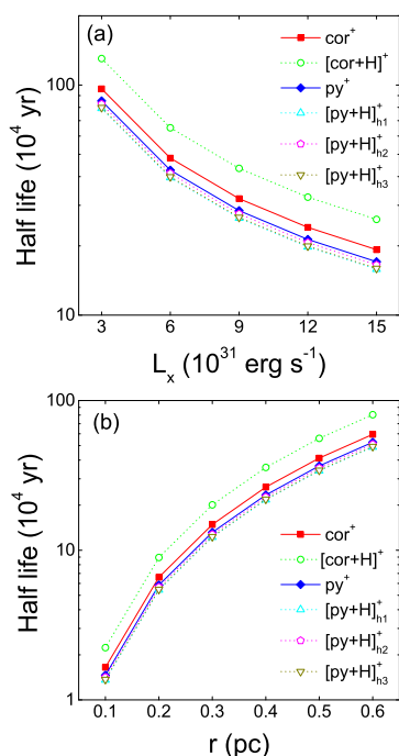
Figure 11. PAH cation half-life for cor^+ , [cor+H]^+ , py^+ and [py+H]^+ as a function of X-ray luminosity L_{X-ray} (a) and as a function of distance from central star to position r (b). (a): r = 0.5 pc; (b): L_{X-ray} = 7 \cdot 10^{31} erg s -1 .
