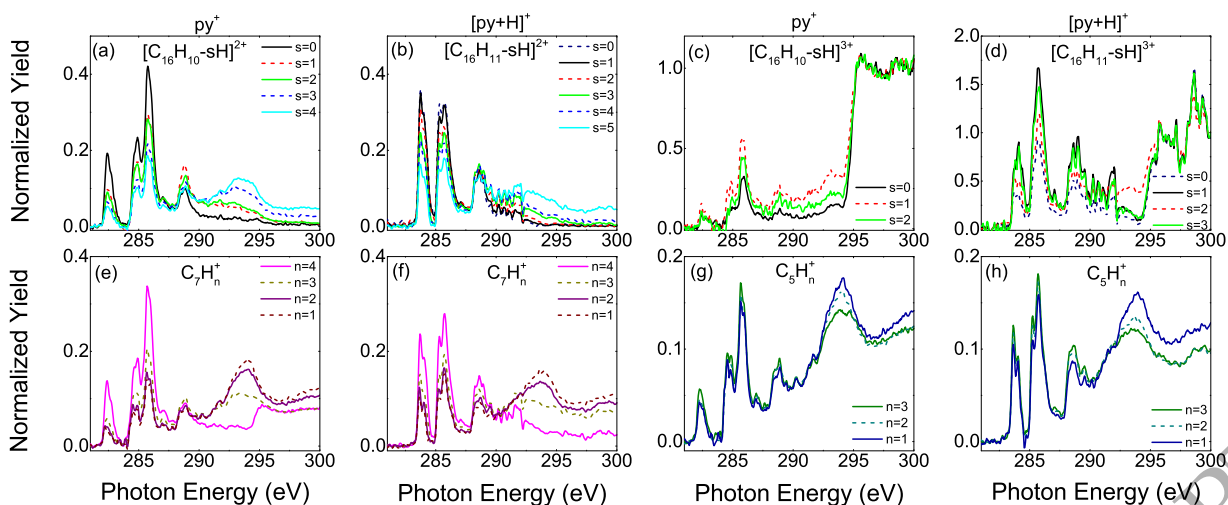
Figure 6. The top row of panels presents NEXAMS data for dicationic and tricationic fragments produced from py^+ and [py+H]^+ . Spectra for non-dissociative single ionization (NDSI) into C_{16}H_{10}^{2+} (a), and into C_{16}H_{11}^{2+} (b) and non-dissociative double ionization (NDDI) into C_{16}H_{10}^{3+} (c), and C_{16}H_{11}^{3+} (d) are shown in black. Spectra associated to loss of s H atoms are shown in color. Dication spectra are normalized to the integral over the excitation region. Trication spectra are normalized to the average yield in the ionization region. The bottom row of panels shows data for the monocationic fragments C_7H_n^+ (e), (f) and C_5H_n^+ (g), (h).
