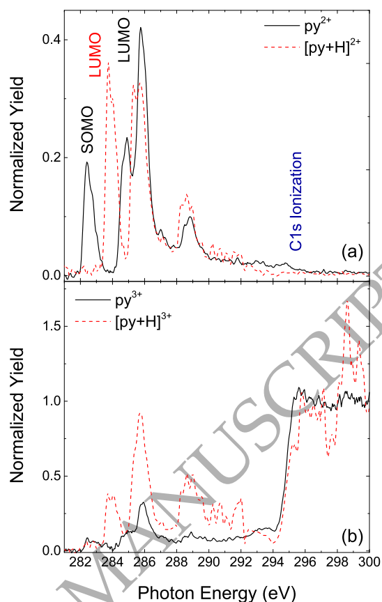
Figure 3. Top panel: NEXAMS data for \text{C}_{16}\text{H}_{10}^{2+} from \text{py}^+ and \text{C}_{16}\text{H}_{11}^{2+} from [\text{py}+\text{H}]^+ (normalized to the integral of the total yields in excitation range). Bottom panel: NEXAMS data for \text{C}_{16}\text{H}_{10}^{3+} from \text{py}^+ and \text{C}_{16}\text{H}_{11}^{3+} from [\text{py}+\text{H}]^+ (bottom panel, normalized to the ionization continuum). Transitions to SOMO and LUMO are indicated. The 1s binding energy is around 295 eV where a threshold-like increase of trication yields is observed.
