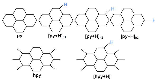
Figure 1. Top row, from left to right: The structures of py, [py+H]_{h1} , [py+H]_{h2} , [py+H]_{h3} . The indices h1, h2 and h3 indicate three different outer edge hydrogen attachment sites for [py+H] . Bottom row, from left to right: The structure of hpy and [hpy+H] . Only 4 hpy outer edge sites can accommodate hydrogen attachment which are symmetrically equivalent.
