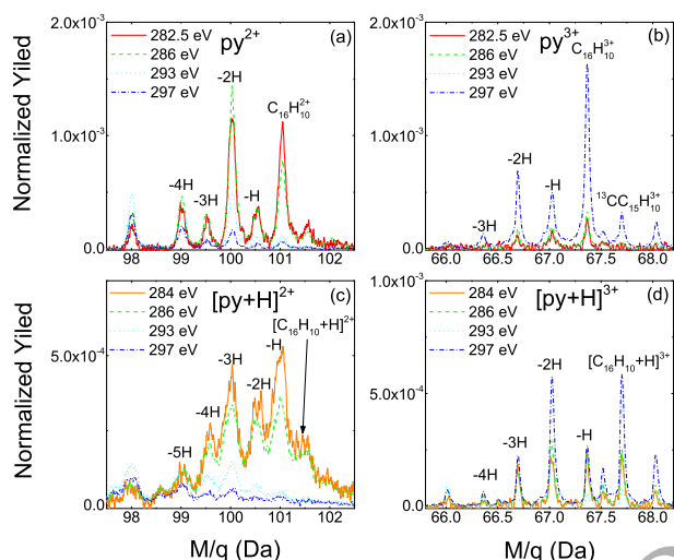
Figure 9. Mass spectra for dicationic and tricationic \text{C}_{16}\text{H}_n formed after soft X-ray photofragmentation of \text{py}^+ (top row of panels) and [\text{py}+\text{H}]^+ (bottom row of panels).
