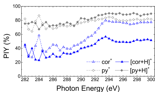
Figure 8. Relative PIY (%) of fragments due to carbon backbone fragmentation of \text{cor}^+ (blue), \text{py}^+ (grey) and their hydrogenated counterparts. The PIY (%) of \text{cor}^+ and \text{py}^+ are indicated by dashed curves while [\text{cor}+\text{H}]^+ and [\text{py}+\text{H}]^+ are displayed by solid curves.
