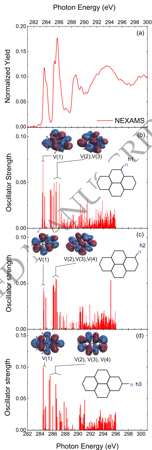
Figure 5. (a): C_5H_3^+ NEXAMS spectrum for [py+H]^+ . (b, c, d) TD-DFT calculated stick spectrum of oscillator strengths for the three different isomers of [py+H]^+ ( [py+H]_{h1}^+ , [py+H]_{h2}^+ and [py+H]_{h3}^+ ). Selected final states are shown as molecular orbitals. Theoretical data has only been calculated up to 296 eV.
