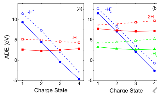
Figure 10. Adiabatic dissociation energies (ADE) for fragmentation channels associated with \text{H}/\text{H}_2/2\text{H} loss as a function of charge state of \text{py}^{q+} (dash curves) and [\text{py}+\text{H}]^{q+} (solid curves). (a) \text{H} loss (squares) and \text{H}^+ loss (circles). \text{H} and \text{H}^+ are lost from the "a" site (see sketch) for \text{py}^{q+} and from the "b" site for [\text{py}+\text{H}]^{q+} . (b) 2\text{H} loss (squares), \text{H}_2^+ loss (circles) and \text{H}_2 loss (triangles) as functions of PAH charge state. 2\text{H}/\text{H}_2/\text{H}_2^+ loss is from the "a" and "b" sites for both \text{py}^{q+} and [\text{py}+\text{H}]^{q+} . All calculations for [\text{py}+\text{H}]^{q+} were all done for the h2 isomer (see Fig. 1), hydrogenated at the "b" site.
