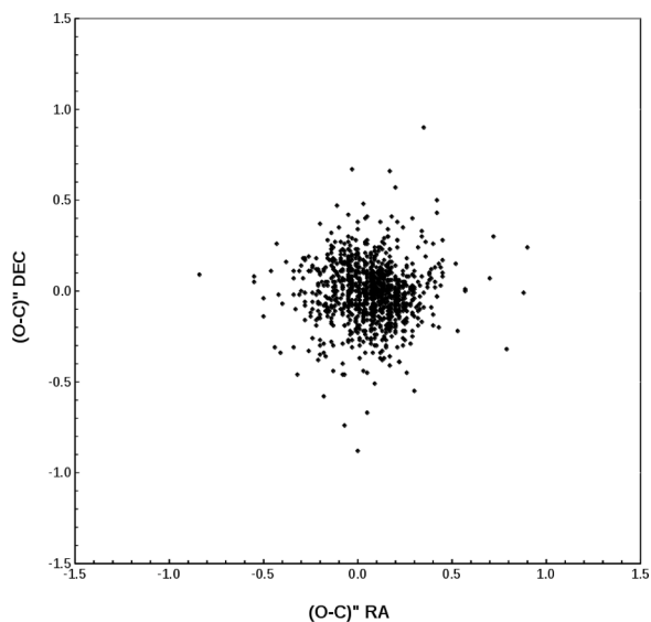
Fig. 5. Observed minus calculated (O-C) residuals for about 300 known numbered asteroids observed during 5/6 Nov 2018. The O-Cs were calculated using the FITSBLINK server ( http://www.fitsblink.net/residuals ).
