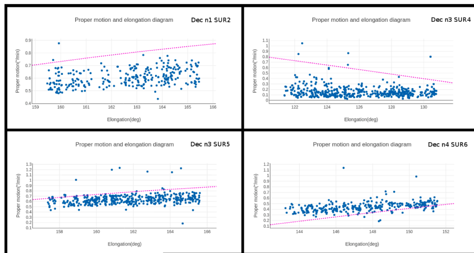
Fig. 7. Samples of the \epsilon - \mu plots classifying possible NEA candidates in entire survey fields observed with the INT during our Dec 2018 NEARBY mini-survey.
