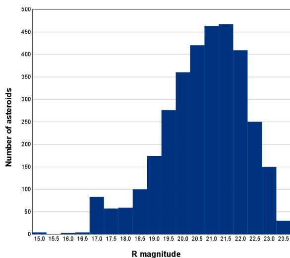
Fig. 6. Sample of histogram plotting the INT photometric survey limits for valid asteroid NEARBY detections (70 WFC fields observed during 2/3 Nov 2018 night).
