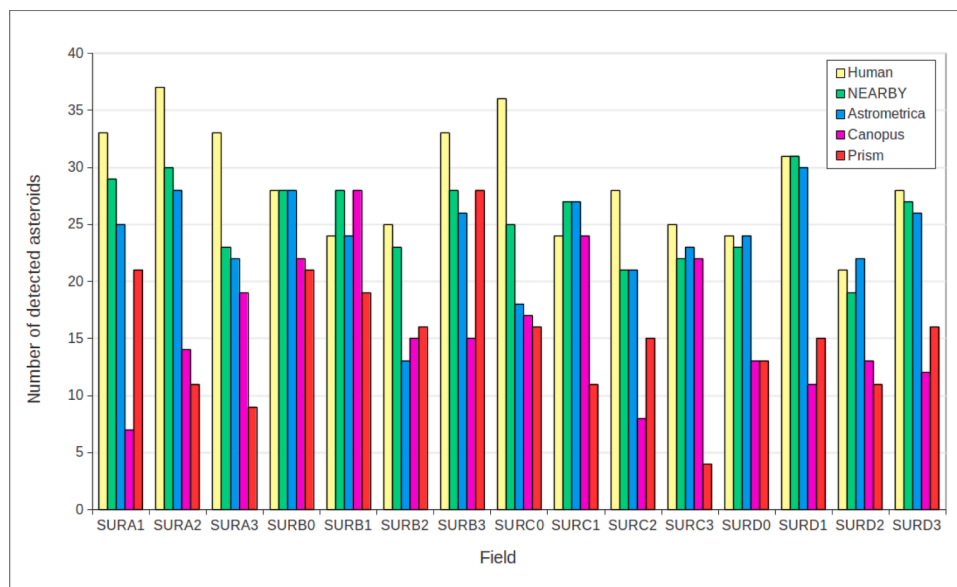
Fig. 8. Comparison between valid NEARBY asteroid detections in the Mar 2017 mini-survey, with results reduced by other similar software and human blink detection.
