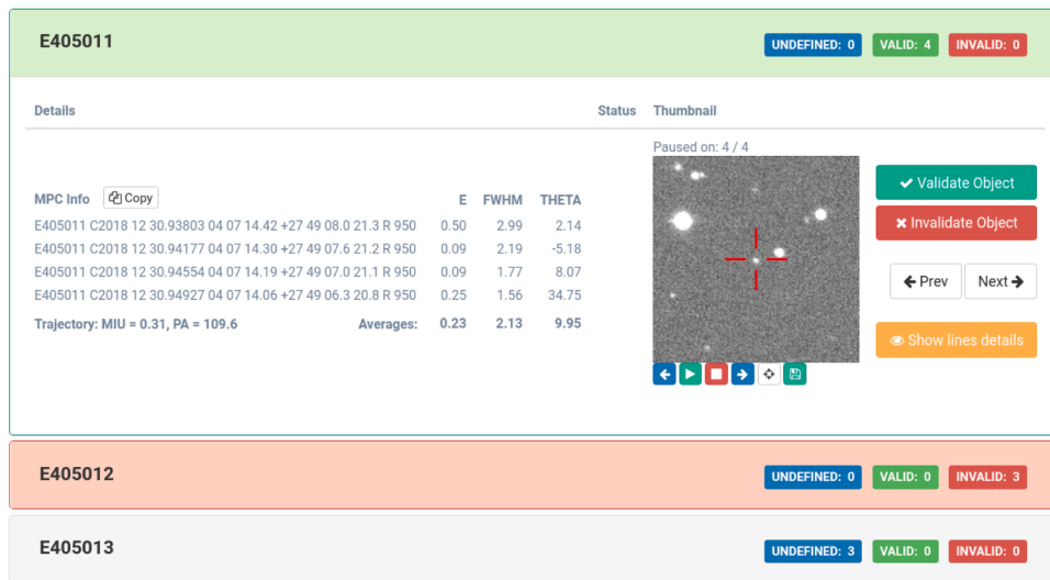
Fig. 1. NEARBY MPC Report interface assisting the reducers to validate moving sources.
