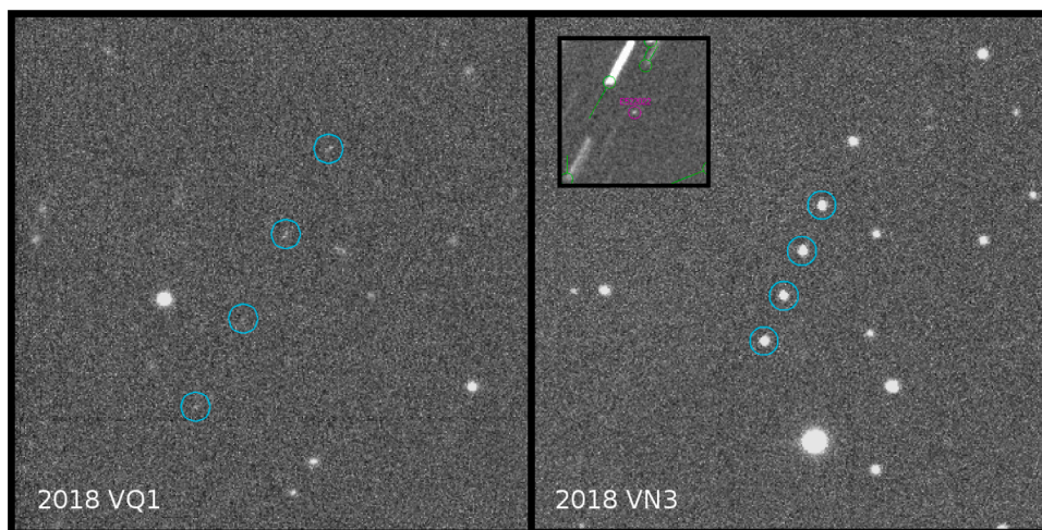
Fig. 3. The first two NEARBY NEA discoveries during the Nov 2018 pilot mini-survey using the Isaac Newton Telescope (INT). The figures match the normal sky orientation, and each field is about 4' \times 4' . Left: 2018 VQ1 discovered by M. Popescu (1 Nov 2018) based on NEARBY reduced images and visual blink in Astrometrica ; Right: 2018 VN3 discovered by C. Boldea (6 Nov 2018) based on NEARBY detection, recovered by L. Hudin using his small 30-cm diam amateur telescope in Cluj-Napoca, Romania (small inset combined track and stack image).
