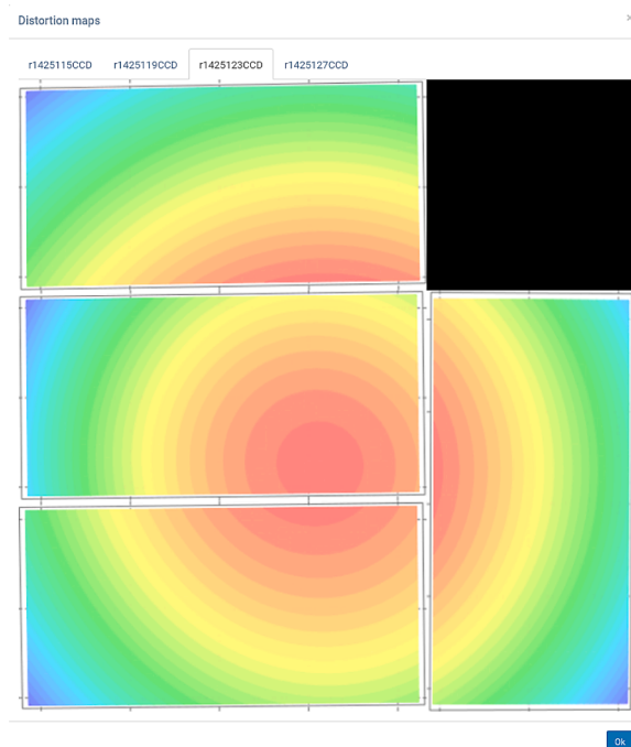
Fig. 4. Typical Scamp distortion map showing the NEARBY reduction of the third image (r1425123 .fit) of the field E557 observed at 5/6 Nov 2018 with the INT/WFC, with the color map mapping slightly different pixel scales.
