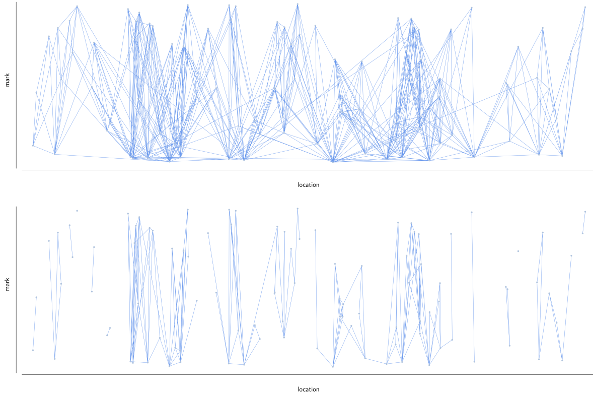
Figure 2: Two simulations for the (rescaled) soft Boolean model on the torus \mathbb{T}_{100}^1 with \delta = 3.5 and \beta = 1 . The first picture was simulated with \gamma = 0.75 , the second one with \gamma = 0.51 .
