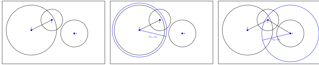
Figure 1: Example for the connection mechanism of the soft Boolean model in two dimensions. The solid lines represent the graph's edges.
