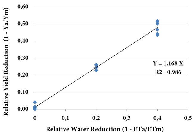
Figure 2: Pearl millet yield response factor (Ky)
