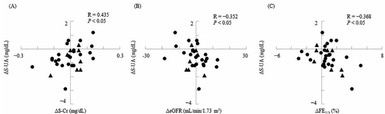
Figure 1. Relationship between \Delta S-UA and \Delta clinical variables. n = 33 . \Delta S-UA and \Delta clinical variables were changes at 6 months from baseline. Men is indicated by circles, women by triangle. S-UA; serum uric acid, S-Cr; serum creatinine, eGFR; estimated glomerular filtration rate, FE_{UA} ; renal fractional excretion of uric acid. All data were analyzed by Pearson's product-moment correlation coefficient.
