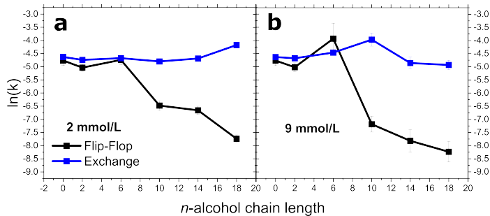
Fig. 3 The alcohol chain length dependence of DMPC intervesicular exchange (blue) and flip-flop (black) at (a) 2 and (b) 9 mmol/L concentrations of alcohols. The standard error is derived from fits iterated by a Levenberg-Marquardt algorithm.
