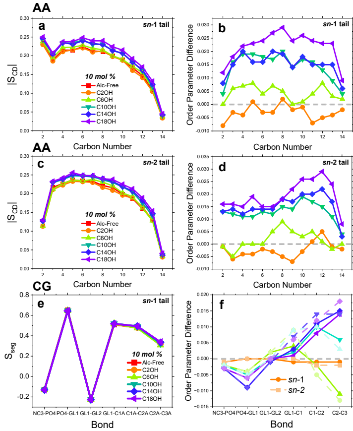
Fig. 7 a) c) Deuterium order parameter of the DMPC alkyl sn -1 and sn -2 tails as a function of n -alcohol chain length. The corresponding b) & d) plots are the order parameter differences between undoped and doped sn -1 and sn -2 tails, respectively. e) Segmental order parameters calculated from CG DLPC (same as DMPC using Martini beads) systems. f) Solid lines and filled symbols are the segmental order parameter difference of sn -1 chains, while transparent dashed lines and symbols are that of sn -2 chains.
