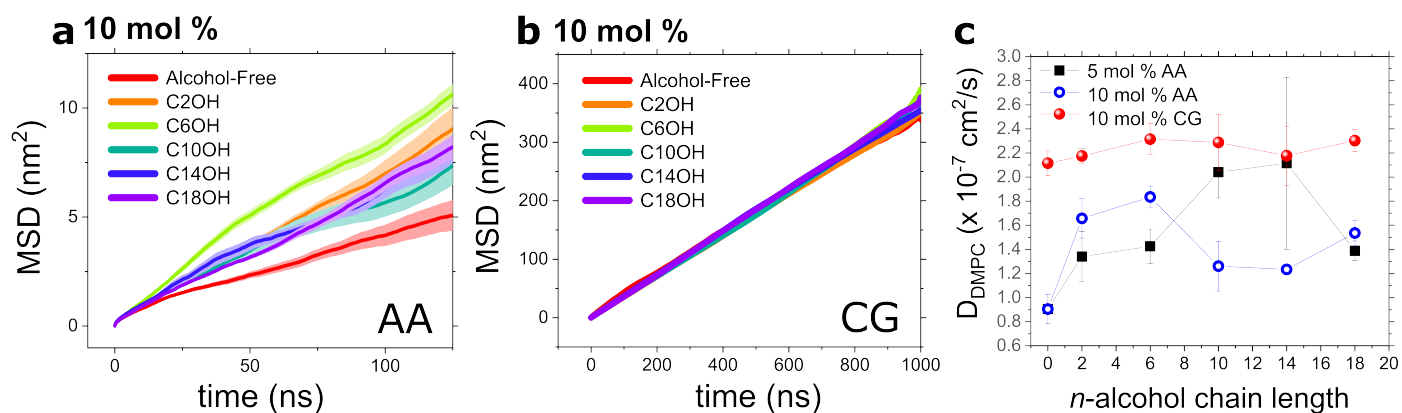
Fig. 8 Mean square displacement plots calculated from a) AA and b) CG simulations of DMPC model bilayers doped with 5 or 10 mol % n -alcohols at 37°C. Linear fits were performed on linear portions of the MSD curves and the resulting lateral DMPC diffusion coefficients within the plane of the lipid bilayer, i.e. perpendicular to the bilayer normal, are presented in c). Errors are estimated from six sub-populations of DMPC molecules for AA values.
