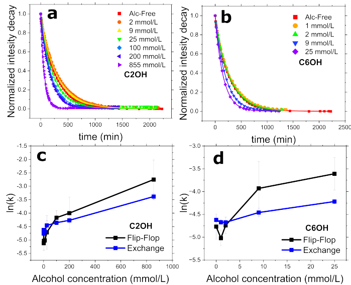
Fig. 2 a) & b) Normalized intensity decay curves of DMPC vesicle mixing under the influence of short-chain alcohols: ethanol (C2OH) and 1-hexanol (C6OH), respectively. Symbols represent the normalized integrated area under each SANS curve at their corresponding time-point; lines are the fits using equation 2 to the decay curves to extract out DMPC flip-flop and exchange rate constants, as seen in c) & d). All measurements were conducted at a temperature of 37°C.
