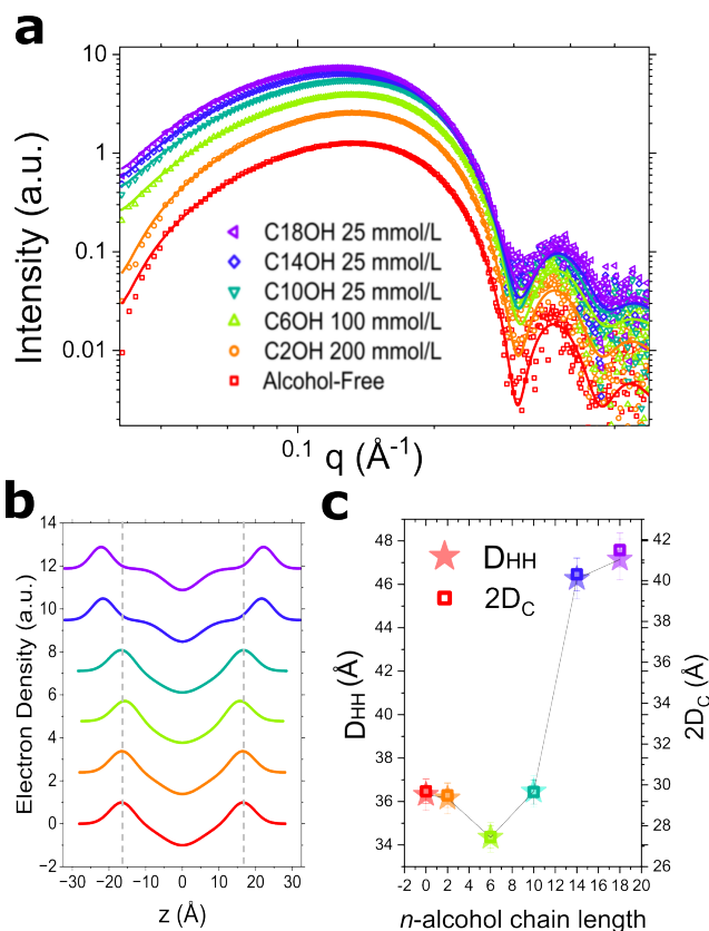
Fig. 4 a) Small angle x-ray scattering curves of DMPC vesicles at 17 mg/mL (21 mmol/L) in 45% D_2O with the inclusion of high concentrations of n -alcohols. Open symbols are the background subtracted data obtained from SAXS; solid lines represent the fits obtained by GAP. b) The electron density profile across the bilayer ( z ) provided by the GAP fit. Note, 0 is the bilayer centre. Relevant bilayer thickness, D_{HH} and 2D_C , are shown in c). Experimental error is estimated to be \leq 2\% as per the scattering density profile model 38 . All measurements were conducted at 37°C.
