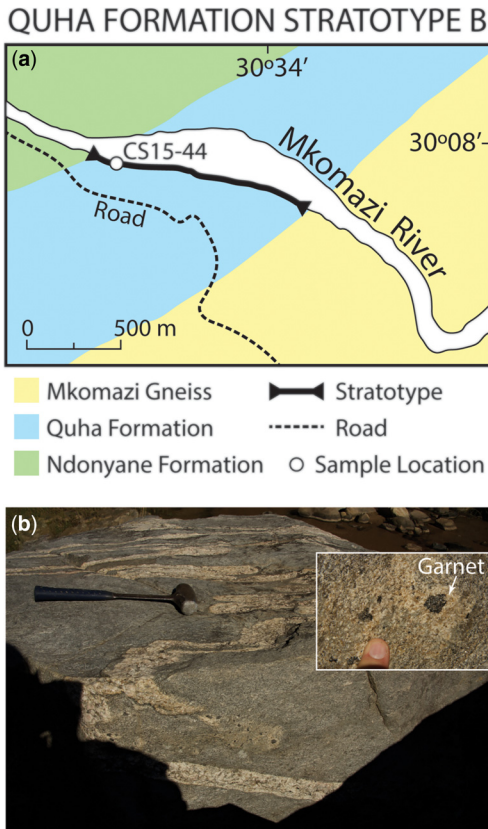
Fig. 2. (a) Simplified geological map of the Quha Formation stratotype B showing the sample locations. (b) Field photograph of the Quha quartzofeldspathic semi-pelitic gneiss with folded leucosomes. Rare garnet porphyroblasts rich in inclusions are visible, with a closer view shown in the inset. The geological hammer is for scale.
