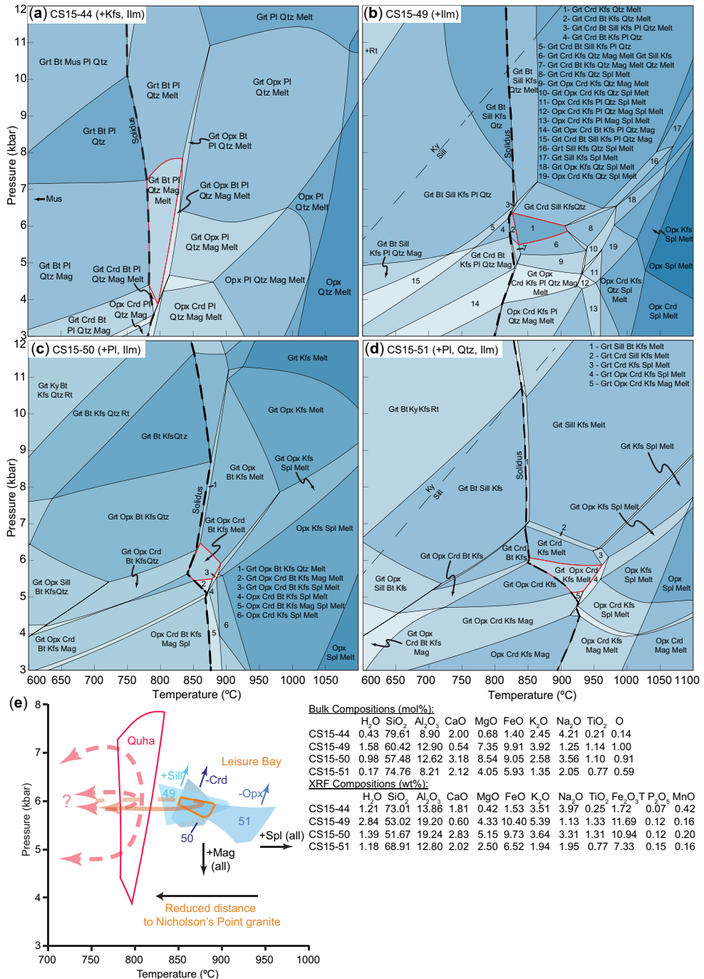
Fig. 9. P - T pseudosections of (a) sample CS15-44 from the Quaha Formation, and (b) samples CS15-49, (c) CS15-50 and (d) CS15-51 from the Leisre Bay Formation. The solidus is highlighted by a black dashed line, with the interpreted peak assemblage outlined in red. (e) P - T summary diagram with potential P - T paths for both the Quaha Formation (red) and Leisre Bay Formation (orange), and the field of overlap between the three Leisre Bay samples (CS15-49–CS15-51). Bulk compositions used in the modelled pseudosections are also listed in mol%, as well as original XRF bulk compositions in wt%.
