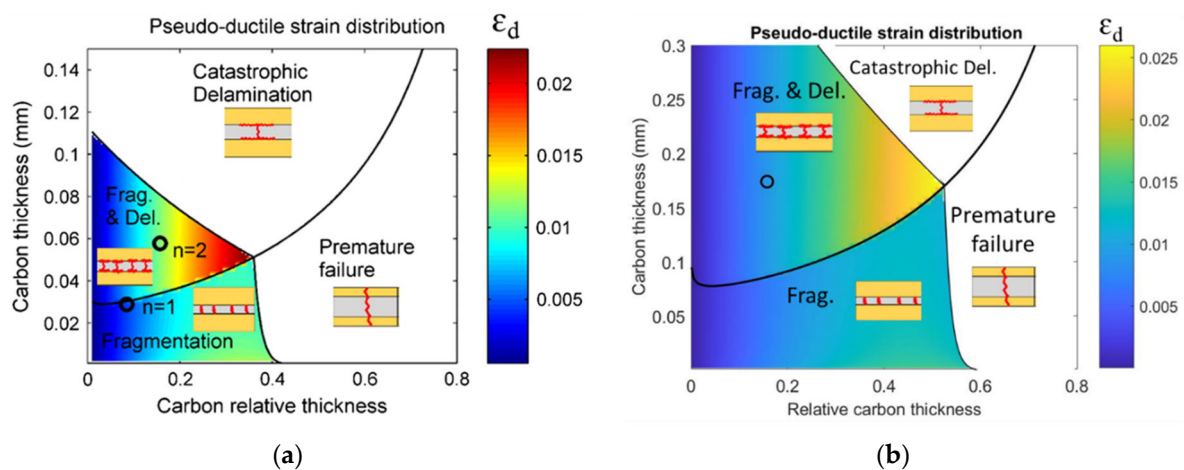
Figure 3. Failure mode maps in the investigated configurations, UD (a) and QI (b).
