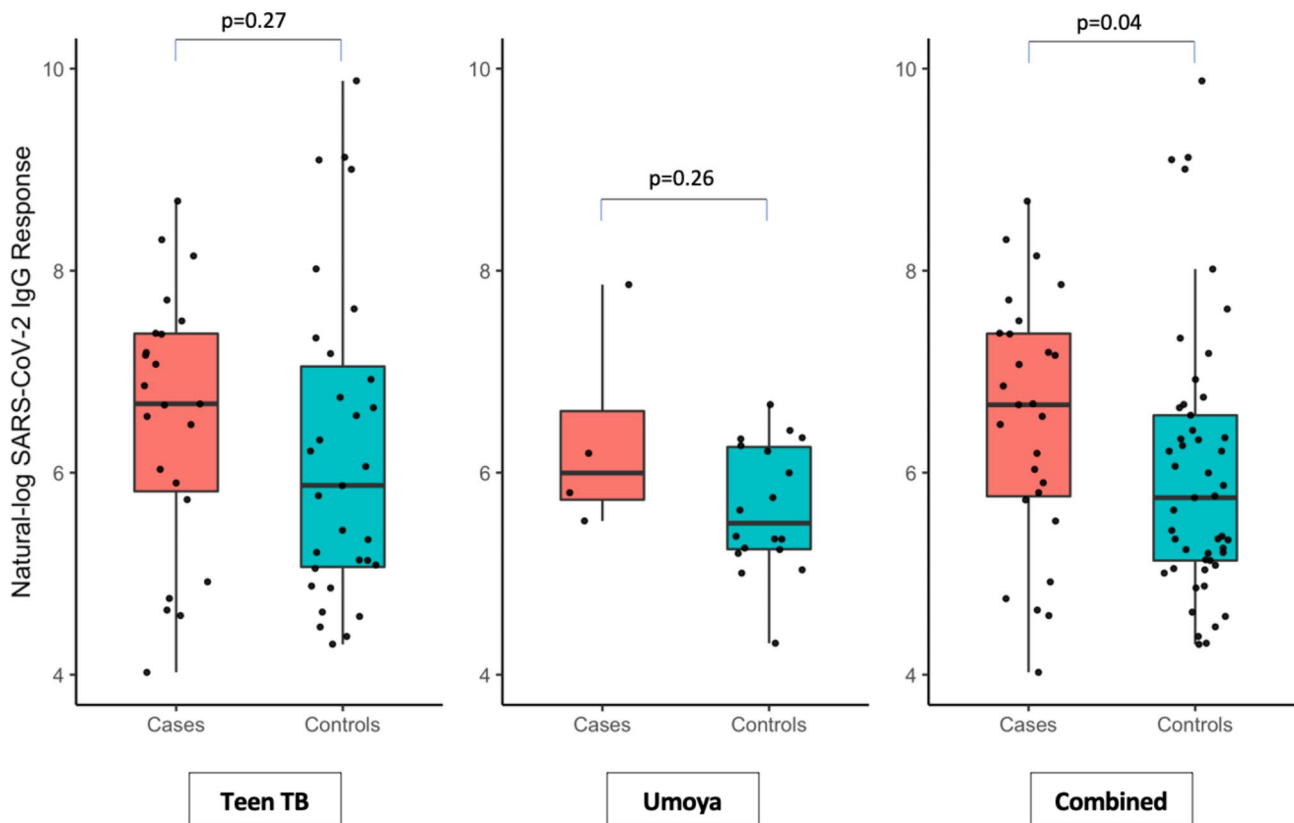
Fig. 2 Log-transformed SARS-CoV-2 IgG response values for SARS-CoV-2 IgG positive cases and controls with accompanying p-value from a Mann-Whitney U-test
