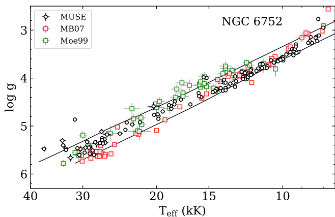
Fig. 12. Kiel diagram showing the position of the stars in NGC 6752 for our MUSE sample (black circle) and for samples taken from the literature (Moni Bidin et al. 2007, red squares and Moehler et al. 1999, green squares).
