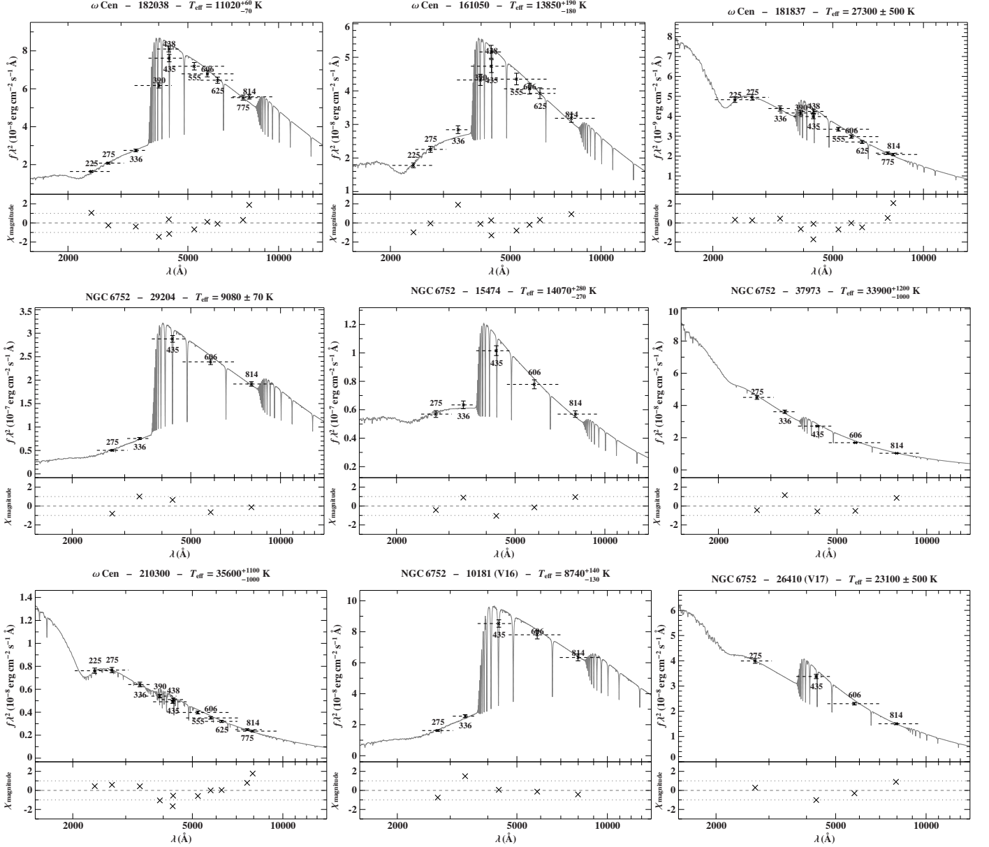
Fig. 6. Examples of photometric (SED) fits with free parameters \Theta and T_{\text{eff}} . On the y-axis, we plot the flux f_\lambda multiplied by \lambda^2 . The best-fit model is plotted in grey while the flux corresponding to the observed magnitude in each filter is indicated along with the central wavelength of the filter. The horizontal dashed lines show the wavelength coverage of each filter. The top panels show the best fits for an A-BHB, B-BHB, and EHB type star in \omega Cen. The middle panels show fits for counterpart stars in NGC 6752. The bottom panels show fits for a blue hook star in \omega Cen, the BSS V16, and the EHB star V17 in NGC 6752. The uncertainty-weighted residuals ( \chi = (\text{mag}_{\text{model}} - \text{mag}_{\text{observed}}) / \text{uncertainty} ) are plotted at the bottom of each fit. The cluster name, star identification number, and resulting T_{\text{eff}}^{\text{SED}} are indicated for each fit.
