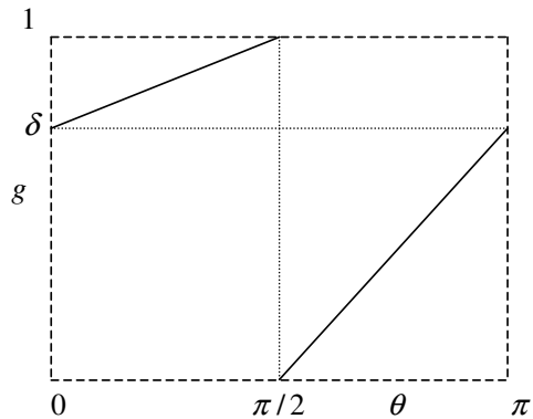
Figure 5: Invertible and discontinuous g -function defined in Eq. (34).
