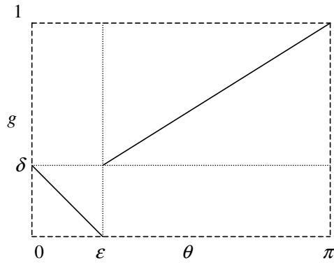
Figure 3: Invertible and discontinuous g -function defined in Eq. (31).
