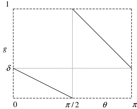
Figure 4: Invertible and discontinuous g -function defined in Eq. (33).
