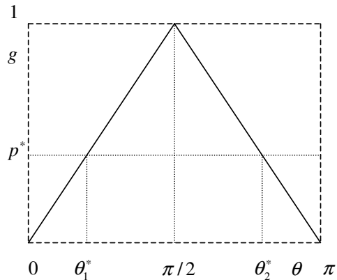
Figure 8: Non-invertible and continuous g -function defined in Eq. (37).
