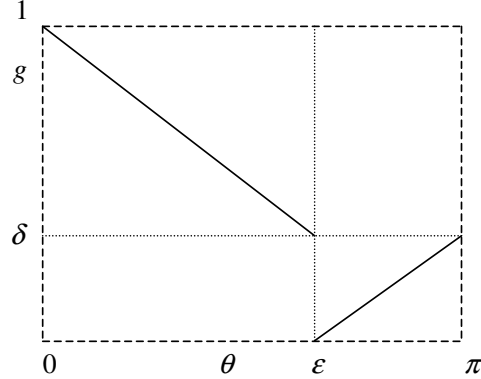
Figure 7: Invertible and discontinuous g -function defined in Eq. (36).
