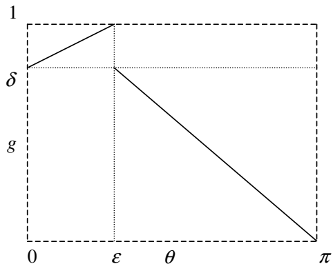
Figure 6: Invertible and discontinuous g -function defined in Eq. (35).
