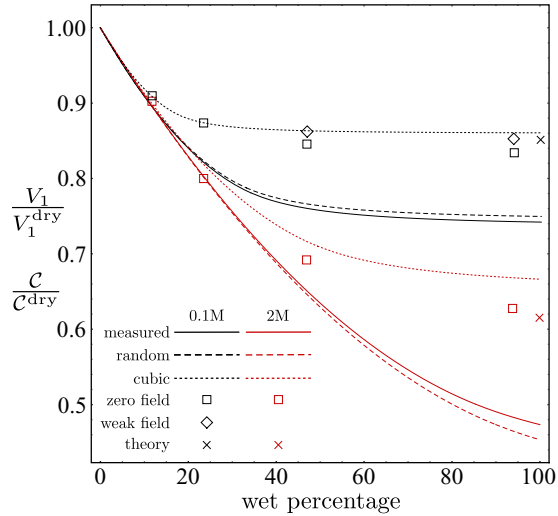
FIG. 9. Normalized particle velocity due to Eq. (74) (lines), and normalized conductivity simulation measurements from Table I (symbols), as a function of wet and dry ratio of species A. All values are normalized by the 0% wet value. Black signifies 0.1 M, red 2 M. The curves indicate the particle velocity, calculated at the average nearest particle separation measured from simulation (solid), and corresponding to random (dashed), and cubic lattice (dotted) configurations. Squares are zero-field conductivity measurements using the Einstein-Helfand formula [Eq. (70)], diamonds indicate weak-field conductivity measurements using the center-of-charge displacement [Eq. (68)], and crosses are the prediction of DHO theory [Eq. (61)].
