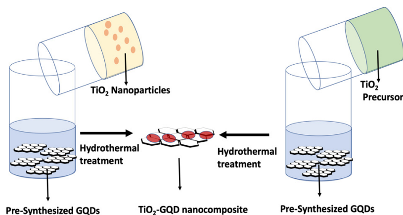
Figure 8. Schematics of TiO 2 -GQDs composite synthesis by hydrothermal method.
