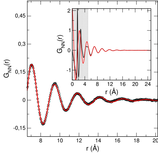
Figure 8. Calculated Bhatia–Thornton NN pair correlation function G_{NN}(r)=r[g_{NN}(r) - 1]=rh_{NN}(r) for P=4.0 GPa (circles), together with a fit from eq. (8) (red curve). The inset shows the entire function with the fit, and the gray zone defines the r -range over which the fit has not been performed.
