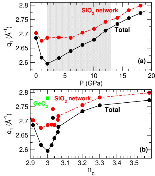
Figure 10. Wave-vector q_1 obtained from the fit of the Bhatia–Thornton pair correlation function rh_{NN}(r) (Fig. 8): (a) q_1(P) , (b) q_1(n_c) . The gray zone represents the reported reversibility window [37]. Green symbol represent experimental data for GeO 2 [93]. The data point for GeSe 2 is out of range (2.10 Å -1 ).
