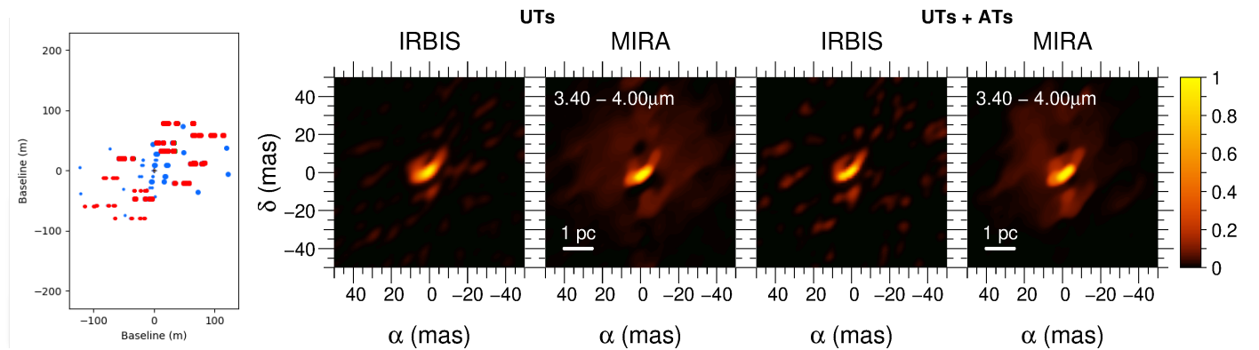
Fig. 20. NGC 1068 and the advantage for the image restoration of combining low frequency AT data with UT data. Left image: u - v coverage, with the AT baselines as blue dots, and the UT baselines are represented as red dots. Two left images: reconstructions are with UT baselines only, while the two right ones combine the baselines of UTs and ATs. The IRBis images are grey reconstructions over the 3.4–4.0 μm interval. The MIRA images are medians of all the 0.1 μm obtained between 3.4 and 4.0 μm.
