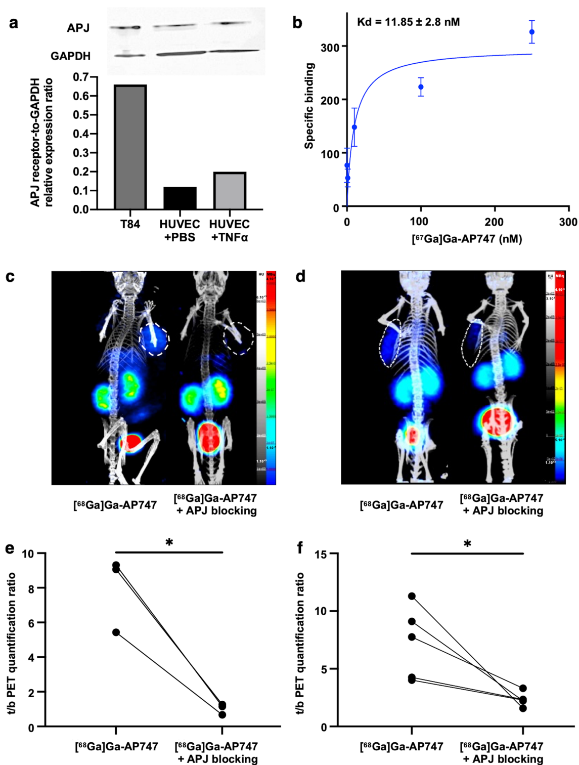
Fig. 3 Semi-quantifications of APJ-to-GAPDH expression ratios by Western blot on human adenocarcinoma T84 cells and HUVECs with or without TNF- \alpha activation ( a ). Saturation binding curve of [ 67 Ga]Ga-AP747 towards APJ receptor on T84 cells ( b ). Representative maximum intensity projections (MIP) images of small animal [ 68 Ga]Ga-AP747 PET/CT in an ectopic mice model of human colon adenocarcinoma, in baseline or APJ-blocking conditions ( c ). Representative MIP of small animal [ 68 Ga]Ga-AP747 PET/CT images of in
