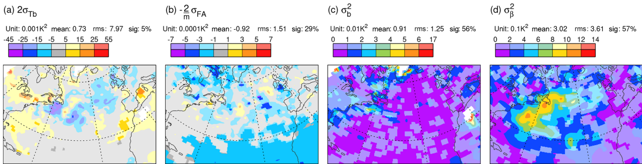
Figure A3. Estimates of the magnitudes of the other terms included in the residual for T500 during the period DJF 2020/2021. (a) Covariance of the analysis bias with the atmospheric state ( \times 2 ). (b) Covariance of the ensemble-mean day-2 forecast and ensemble-mean analysis ( \times -2 ). (c) Variance of the analysis bias. (d) Variance of the day-2 forecast bias (relative to analysis). Note that the units differ widely between panels. Statistically significant values are shown with more saturated colours. Area means (for the area displayed) are indicated at the top of each panel (e.g. “sig: 29 %” means that 29 % of the area is significant at the 5 % significance level). Please see main text for further details.
