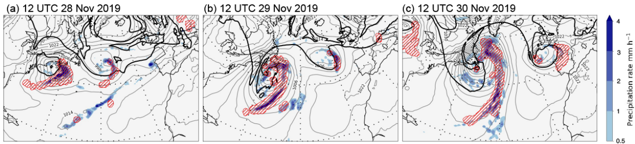
Figure 1. Synoptic overview, based on ERA5 reanalyses, of a North Atlantic cyclogenesis event at 12:00 UTC on (a) 28 November, (b) 29 November, and (c) 30 November 2019. Shown are PMSL (grey contours at intervals of 4 hPa), surface precipitation accumulated over the previous hour (colour shading, in \text{mm h}^{-1} ), the P_{315} = 2 PVU contour indicating the tropopause on 315 K (thick black contour), and the WCB ascent region (red hatching). WCBs are identified as 48 h trajectories that ascend from the lower troposphere by more than 600 hPa (e.g. Wernli and Davies, 1997; Madonna et al., 2014), and the ascent region corresponds to the envelope of the horizontal positions of all WCB trajectories, initialized every 6 h, that are located between 800 and 500 hPa at the indicated time (corresponding approximately to their mid-ascent time).
