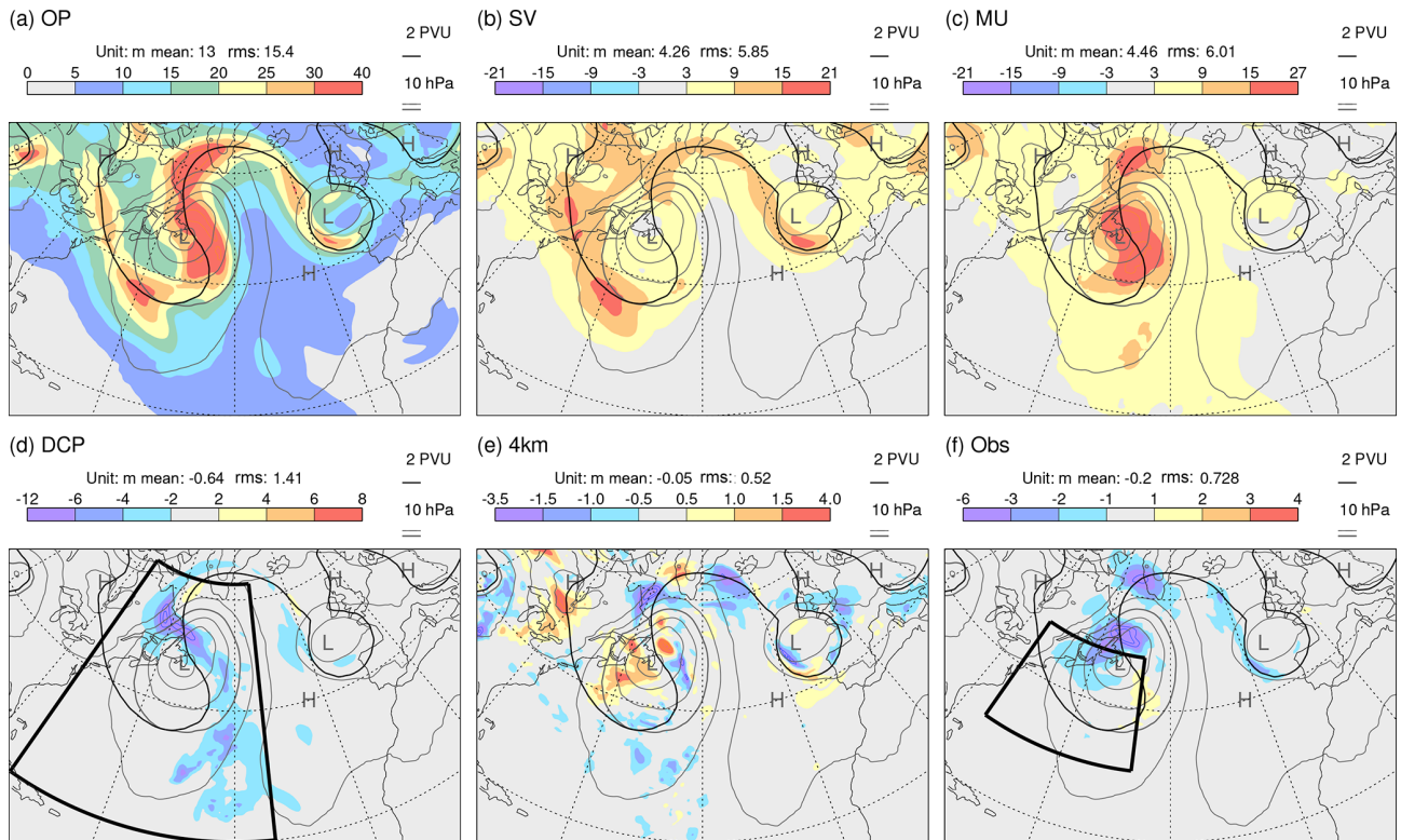
Figure 9. Sensitivity results showing day-2 Z250 spread (shaded) from ECMWF ensemble forecast experiments initialized at 12:00 UTC on 28 November 2019. (a) Total spread for the near-operational configuration OP. (b–f) Differences in spread between experiments which highlight the impacts of (b) including initial singular vector perturbations, (c) including the model uncertainty representation, (d) including the parameterization of deep convection in the indicated region [75–34° W, 20–63° N], (e) an increase in model grid resolution to ~4 km, and (f) the assimilation of observations in the indicated region [75–47° W, 30–49° N]. Note that the shading interval varies across the panels. Contours extend the shading scheme, with the same interval. In these cases, the most extreme values are indicated at the ends of the colour bar. Mean values and rms values, integrated over the area shown, are indicated above each panel. Also shown in each panel are the PMSL (grey contours, with interval 10 hPa and the 1000 hPa contour shown more thickly) and PV = 2 PVU on the 315 K isentropic from the unperturbed EDA analysis.
