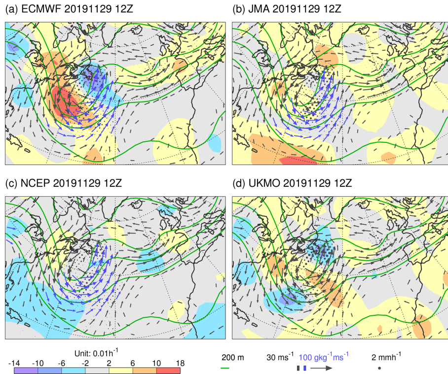
Figure 3. Growth rate LGR_Z for Z250 for TIGGE models (shaded), centred at 12:00 UTC on 29 November 2019. Note that orange contours extend the shading scheme with the same interval, where required. In these cases, the most extreme values are indicated at the ends of the colour bar. Also shown, for the unperturbed ensemble members, are Z250 (green contours) and v_{850} (vectors, which are plotted blue if the moisture flux at 850 hPa exceeds 100 \text{ g kg}^{-1} \text{ m s}^{-1} ). Ensemble mean precipitation is indicated by black dots, with a radius proportional to the precipitation rate up to the maximum size at 2 \text{ mm h}^{-1} . The models shown are from (a) ECMWF, (b) JMA, (c) NCEP, and (d) UKMO as discussed in Sect. 2.2.
