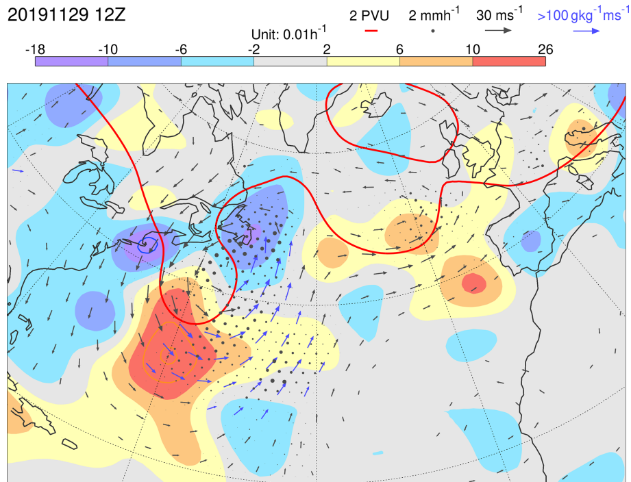
Figure 2. Growth rate LGR_p for P315 in EDA background forecasts (shaded), centred at 12:00 UTC on 29 November 2019. Note that orange and blue contours extend the shading scheme, with the same interval. In these cases, the most extreme values are indicated at the ends of the colour bar. Also shown, for the unperturbed EDA member, are P315 = 2 PVU (red contour) and v850 (vectors, which are plotted blue if the moisture flux at 850 hPa exceeds 100 \text{ g kg}^{-1} \text{ m s}^{-1} ). The ensemble mean precipitation is indicated by black dots (with a radius proportional to the precipitation rate up to the maximum size at 2 \text{ mm h}^{-1} ).
