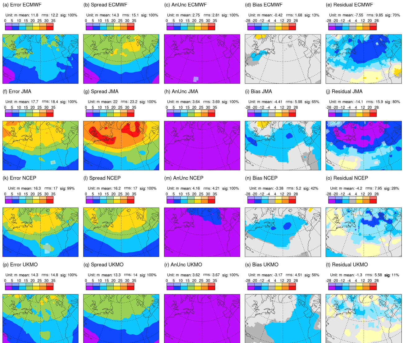
Figure 5. Square roots of terms in the extended error–spread budget Eq. (1) for Z250 based on all day-2 forecasts verifying in DJF 2020/2021. Data come from the TIGGE archive for ECMWF (top row), JMA (second row), NCEP (third row), and UKMO (bottom row) ensembles. Note that the bias and residual, which can take positive and negative values, are shaded with a different interval to the other terms. Statistically significant values are shown with more saturated colours. Area means (for the area displayed) are indicated at the top of each panel (e.g. “sig: 85 %” means that 85 % of the area shown is significant at the 5 % significance level, using an auto-regressive AR(1) model to take account of serial correlation).
