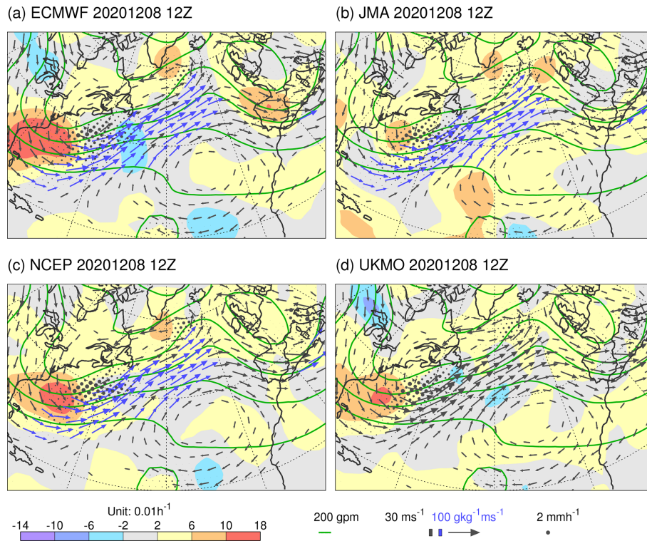
Figure 4. As Fig. 3 but centred at 12:00 UTC on 8 December 2020. This situation also corresponds to an event of cyclone intensification off the North American east coast associated with a WCB.
