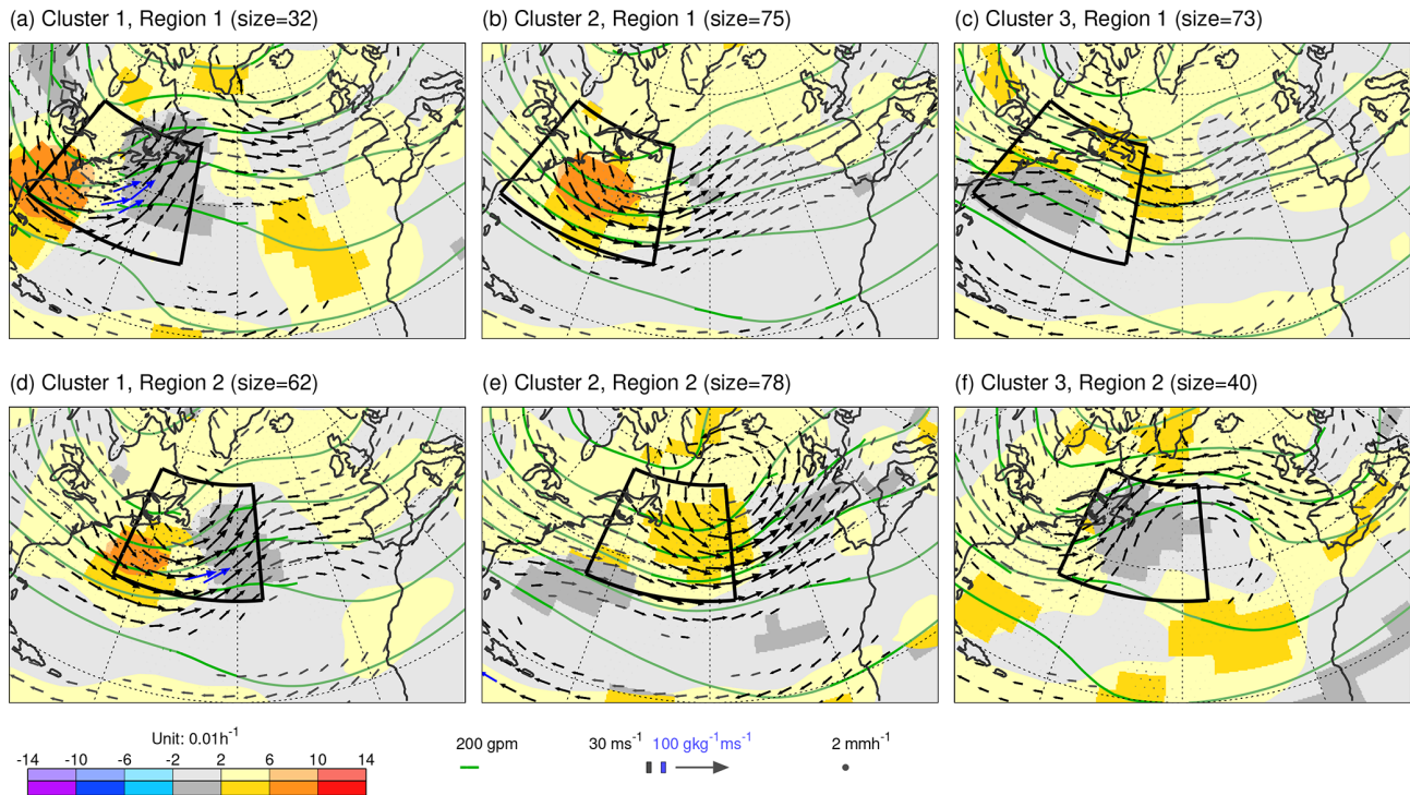
Figure 6. Means over the date/times for the three clusters obtained from K -means clustering in the first (a–c) and second (d–f) region on the fields of Z250 (contours), u850 and v850 (vectors) from ECMWF control (unperturbed) forecasts at step 0, and ensemble mean 12 h accumulated precipitation (dots) valid (or end of accumulation) at 00:00 and 12:00 UTC within the period DJF 2020/2021. The two clustering regions are indicated by the black borders in each panel. Although not used in the clustering, shading shows the corresponding mean 12 h uncertainty growth rate LGR_Z for Z250 . Vectors are coloured blue when the humidity flux at 850 hPa exceeds 100 \text{ g kg}^{-1} \text{ m s}^{-1} . More saturated shading, contours, vectors and dots indicate statistical significance at the 5% level (not accounting for autocorrelation due to the discontinuous nature of date/times in each cluster).
