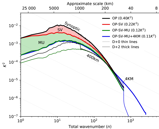
Figure C1. Spectra of ensemble T500 variance for the indicated experiments, summarized in Fig. 8. Spectra show the variance of the ensemble filtered on total wavenumber n for global spherical harmonics. The approximate scale of each harmonic is indicated on the top x axis (this relates to a half wavelength assuming equal zonal and meridional wavenumbers). Thin lines show initial time, and thick lines show day 2. The red, green, and blue shaded regions indicate the impacts at day 2 of including initial singular vector (SV) perturbations, model uncertainty (MU) representation, and increasing the grid-point resolution of the forecast model to \sim 4 km, respectively. Diagonal dotted lines are contours of variance contribution per linear unit length on the x axis, with contour value proportional to the y intercept. Total variance for each experiment is indicated in parentheses in the key.
