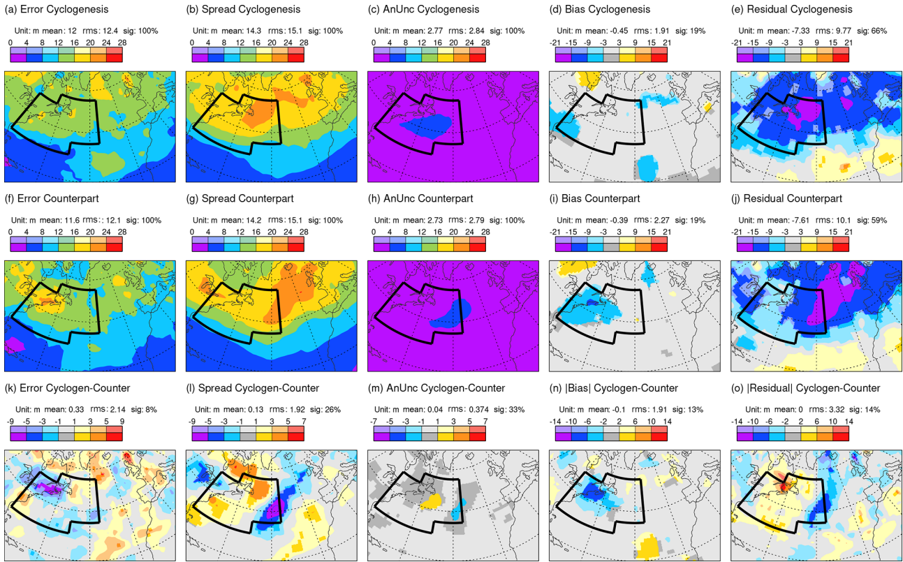
Figure 7. As Fig. 5 but separately for the cyclogenesis composite date/times (top) and the non-cyclogenesis counterpart composite date/times (middle), for forecasts that start two days prior to the cluster classifications. The bottom row shows cyclogenesis minus counterpart. Note that differences in absolute bias and residual are shown, so that blue (red) colours anywhere on the bottom row show where results for the cyclogenesis composite are better (worse) than for the counterpart. The union of the two clustering regions is indicated by the black border.
