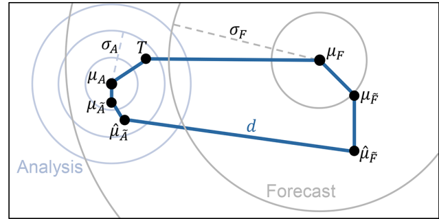
Figure A1. Key concepts in the evaluation of ensemble error–spread reliability. The departure d is the difference between the ensemble mean of the forecast \hat{\mu}_{\tilde{F}} and the ensemble mean of the verifying analysis \hat{\mu}_{\tilde{A}} . The forecast and analysis ensembles can be considered as finite samplings of underlying distributions with (mean, variance) = (\mu_{\tilde{F}}, \sigma_{\tilde{F}}^2) and (\mu_{\tilde{A}}, \sigma_{\tilde{A}}^2) , respectively. Circles depict the hypothetical forecast and analysis distributions with (mean, variance) = (\mu_F, \sigma_F^2) and (\mu_A, \sigma_A^2) , respectively, that would be created with a perfect model (but with imperfect/incomplete observational information). The truth is indicated by a T . See the main text for further discussion.
