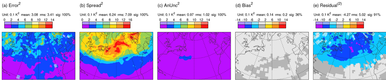
Figure A2. Extended error–spread budget (squared terms) for DJF 2020/2021 for T500 on day 2 from ECMWF ensemble forecasts. Statistically significant values are shown with more saturated colours. Area means (for the area displayed) are indicated at the top of each panel (e.g. “sig: 85 %” means that 85 % of the area is significant at the 5 % significance level).
