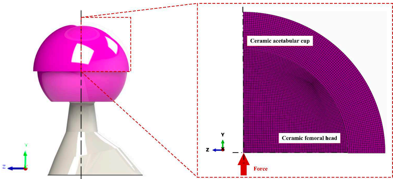
Figure 1. Finite element model of ceramic-on-ceramic coupling.
