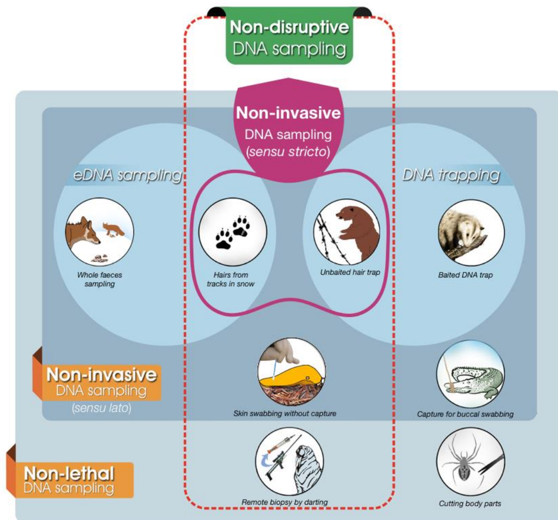
Figure 3. The relationship between non-disruptive, non-invasive and non-lethal DNA sampling methods. Non-invasive DNA sampling sensu stricto corresponds to the definition given by Taberlet et al. (1999), Non-invasive DNA sampling sensu lato corresponds to the medical definition (Miller & Keane, 1983). Pictograms represent a non-exhaustive list of examples for which references are given below. From left to right and top to bottom: whole faeces sampling for species that use faecal territory marking (Modave et al. , 2017), hairs collected in snow (Cullingham et al. , 2016), hairs collected with unbaited barbed wire (Karamanlidis et al. , 2014), DNA trap baited to attract animals (Duenas et al. , 2015), skin swabbing in the field without capture (Morinha et al. , 2014), capture of reptiles for buccal swabbing
