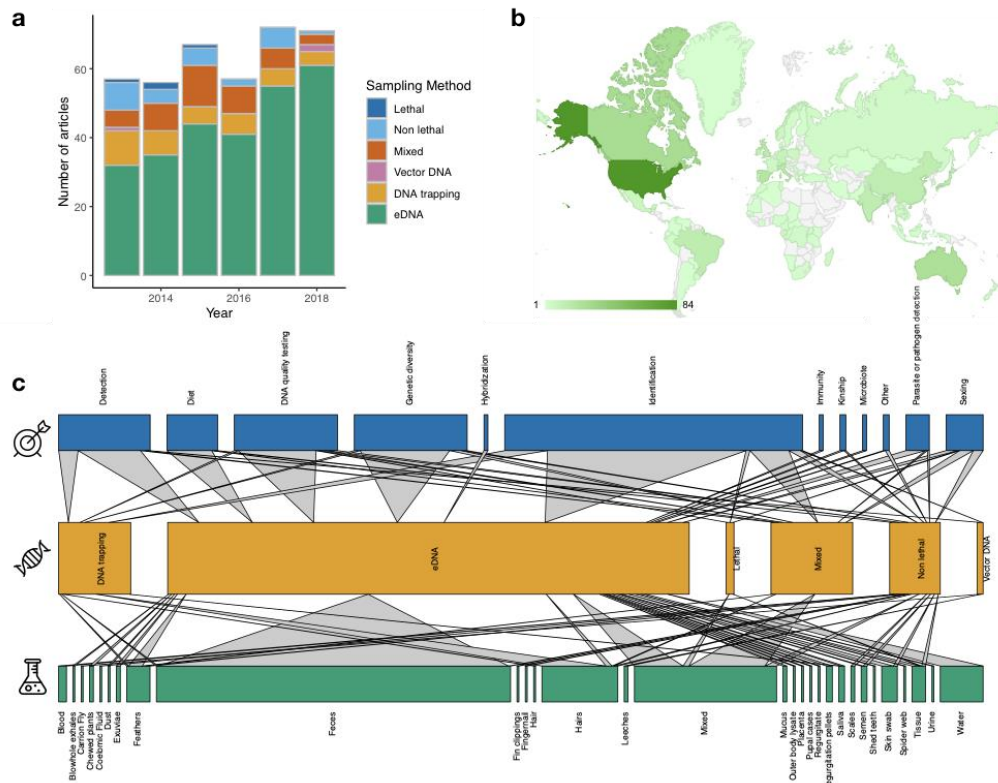
Figure 1. Summary statistics of the literature review on the use of “non-invasive DNA sampling” between January 2013 and December 2018 (n=380). a: Number of articles in relation to the sampling method used between 2013 and 2018. b: Countries of origin of the samples analysed in the reviewed papers. Countries in grey were not represented in our review, countries coloured in various shades of green provided samples for 1 to 84 of the reviewed papers (see in-graph legend for colour scale). c: Bipartite network of the main aim of the studies in blue, the type of sampling method used in orange (see Table 1 for definitions) and the nature of the samples collected in green. The horizontal width of the rectangles is proportional to the number of articles in each category.
