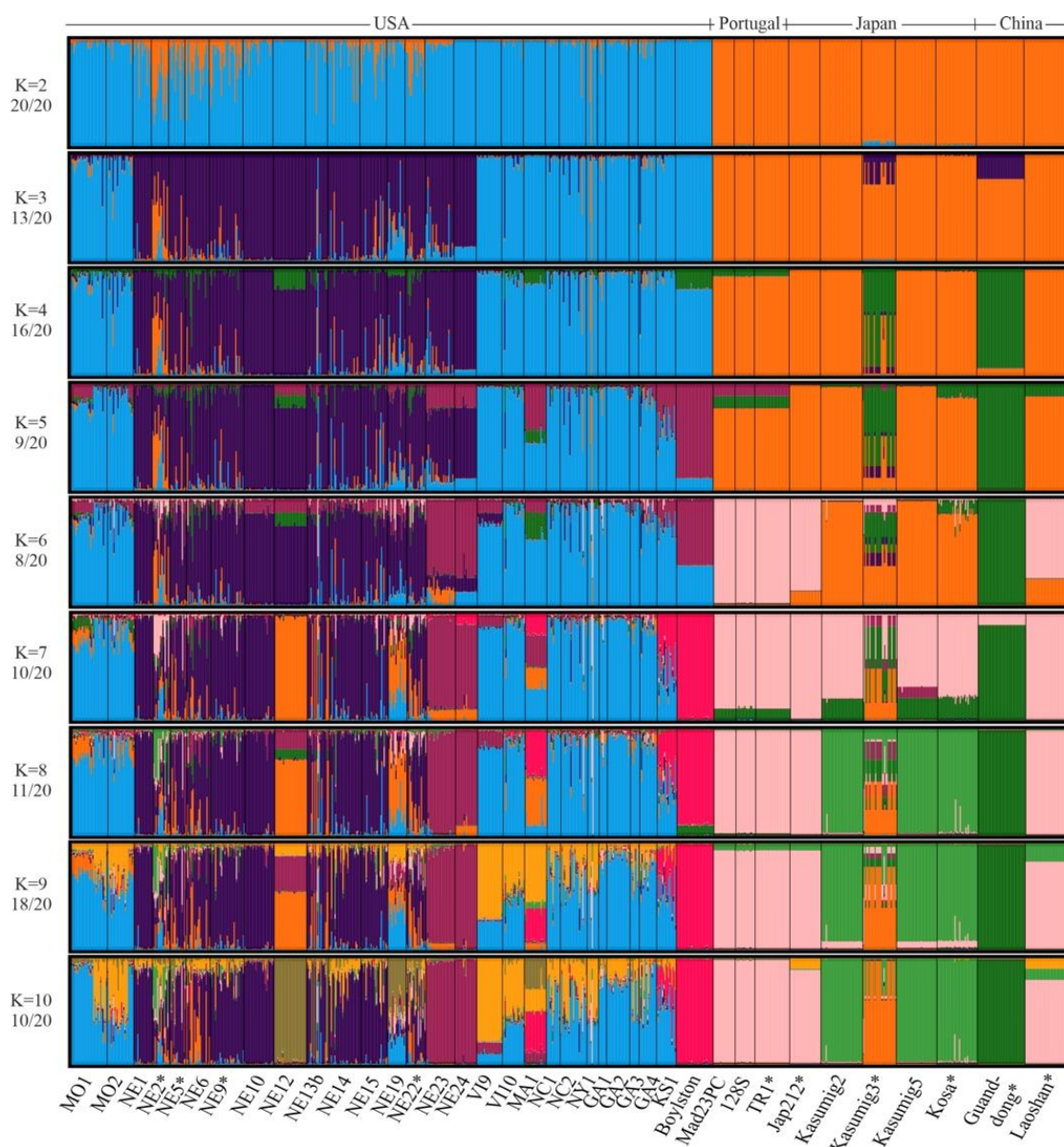
Figure 2: Genetic structure of the pinewood nematode samples used in this study. Bar plots of the coefficients of co-ancestry obtained in STRUCTURE analyses with several values of K. Each bar corresponds to one individual nematode and each cluster is represented with a particular color. The major clustering patterns are shown (see Figure S6B for the minor ones, when applicable). “*” indicates that the corresponding site sample was used in the ABC analyses.
