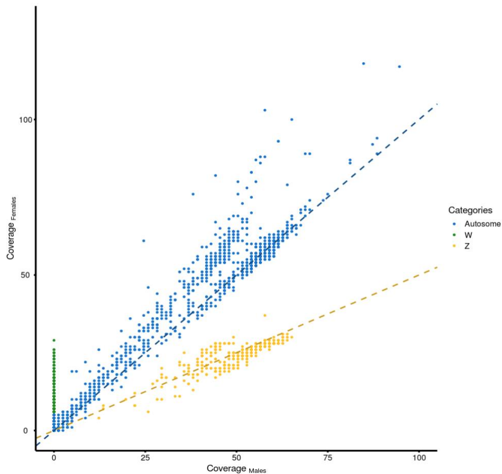
Figure 2. Identification of Z and W scaffolds using coverages of male and female individuals. Normalized sum of median per-site coverage of trimmed reads over the five males (x-axis) and seven females (y-axis). Values were only calculated for scaffolds longer than 10-Kb. Linear regressions for slope=1 (blue) and slope=0.5 (yellow) are shown. Scaffolds were assigned following the decision rule described in the material and methods section.
