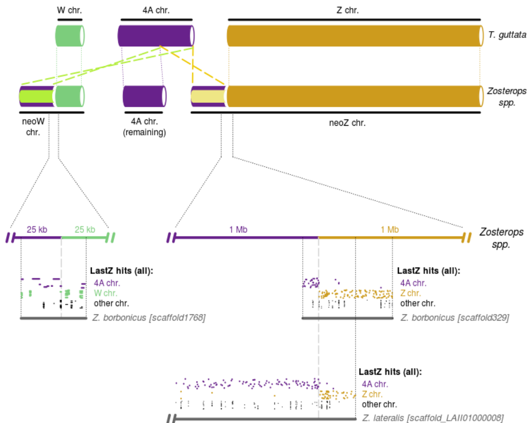
Figure 4. Fine-scale genome architecture of the Sylvioidea neo-sex chromosomes. Original W and Z and autosomal 4A chromosomes are shown in green, yellow and purple, respectively. Translocated regions of the ancestral 4A chromosome (neoW-4A and neoZ-4A) are shown with a purple outline. LASTZ hits on scaffold supporting the chromosomal breakpoints are shown using the same color code. For ease of illustration, coordinates on the Z and 4A chromosomes are reversed (i.e. the white disk represents the beginning of the T. guttata chromosome sequence).
