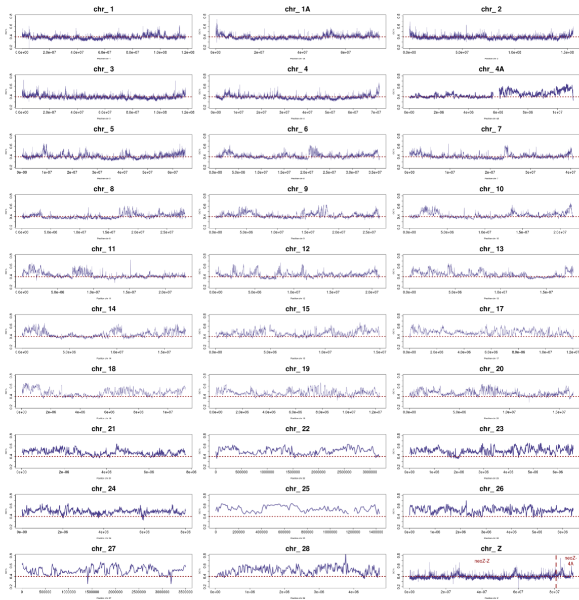
Figure S7. Variation in G+C content along 30 Z. borbonicus chromosomes. The red dotted line indicated the median GC value over non-overlapping 10kb sliding windows for scaffolds assigned to chromosomes only. As expected, strong departures from this median values are observed on minichromosomes.
