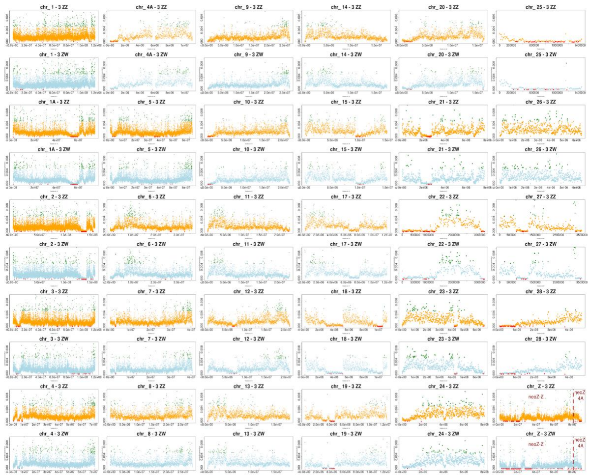
Figure S5. Nucleotide diversity variations along 30 Z. borbonicus chromosomes as estimated using genetic information from three males ( \pi males, orange) and three females ( \pi females, light blue). For each dataset, top 2.5% and bottom 2.5% of \pi values among windows scanning all chromosomes are shown in green and red, respectively. The chromosomal breakpoint on the neoZ chromosome is shown with a red line.
