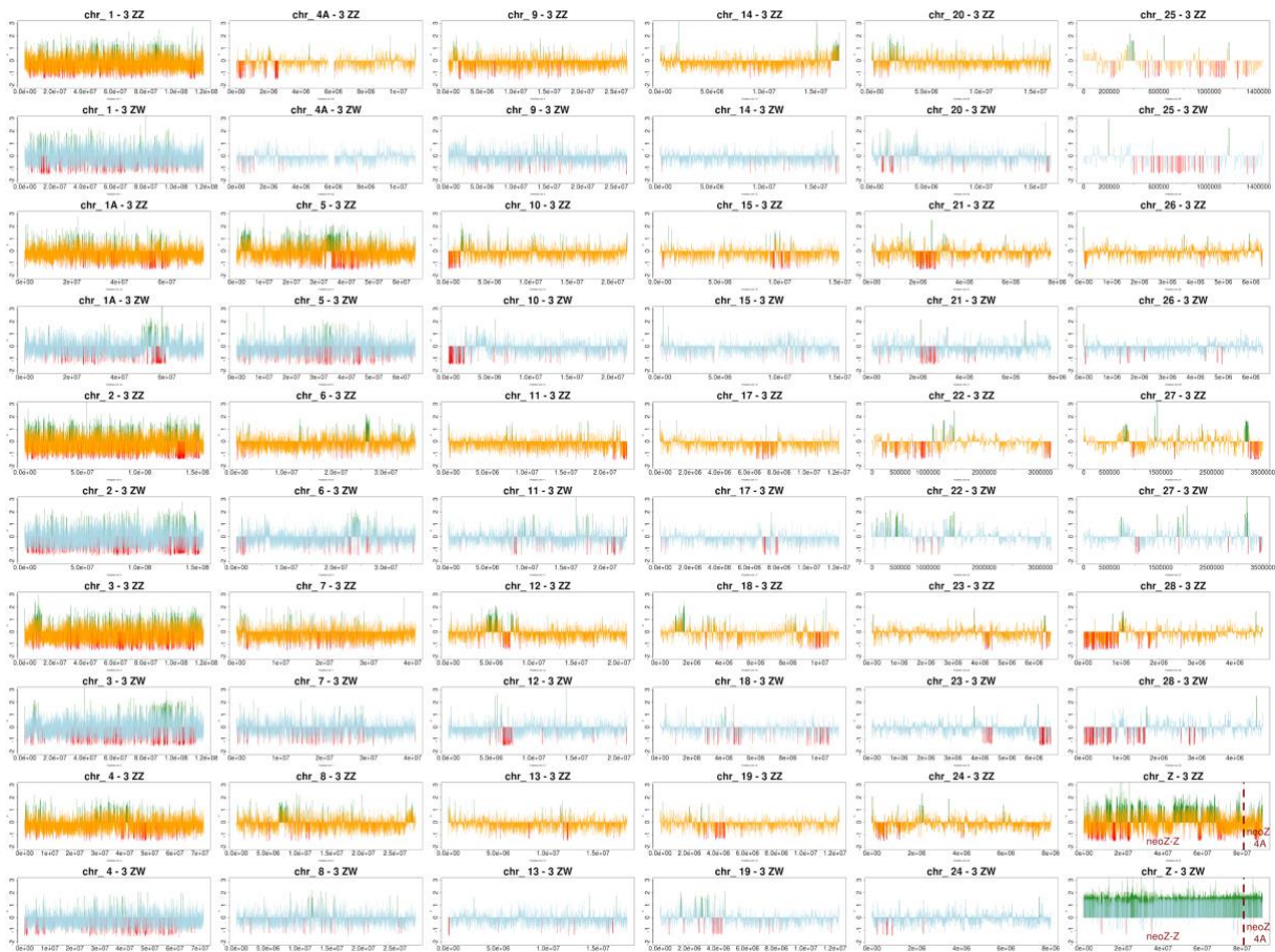
Figure S6. Tajima's D variations along 30 Z. borbonicus chromosomes as estimated using genetic information from three males (orange) and three females (light blue). Top 2.5% and bottom 2.5% of D values among windows scanning all chromosomes are shown in green and red, respectively (baseline for D=0 ). The chromosomal breakpoint on the neoZ chromosome is shown with a red line.
