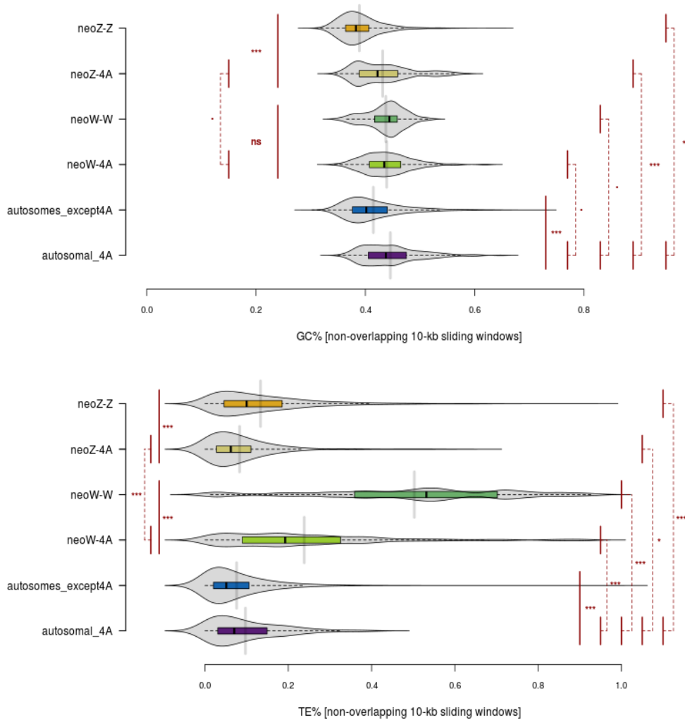
Figure 8. Variation in GC (top) and TE (below) contents between chromosomes. GC and TE contents were estimated along the whole genome using non-overlapping 10-kb sliding windows. Means were compared using t-tests (pairwise comparisons between chromosome sets, without corrections for multiple testing). Thresholds: . < 0.1, * < 0.05, ** < 0.01, *** < 0.001
