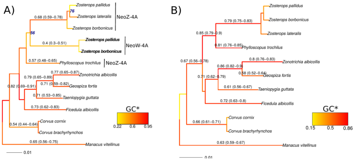
Figure 9. Phylogenetic relationships and estimation of GC equilibrium (GC*). A) Estimation using the 17 genes coded by the translocated region of the ancestral chromosome 4A (0-9.6 Mb). Bold font indicates NeoW-4A sequences. B) Estimation using the 79 genes coded by the non-translocated region of the ancestral chromosome 4A (9.6-20.7 Mb). Branch color and numbers above branches indicated GC*, mean and 95% confidence interval obtained by bootstrap are in parenthesis. Number in blue in front of the node indicates ultra-fast bootstrap values lower than 100%.
