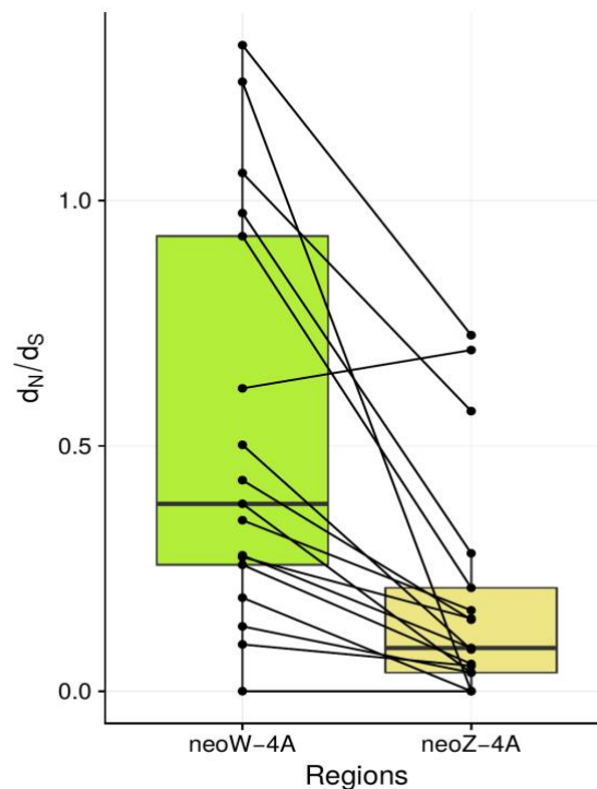
Figure 7. The d_N/d_S ratios of the neoW-4A and neoZ-4A copies (gametologs) of the Zosterops borbonicus genomes. For each gene, horizontal lines linked values of the two gametologs.
