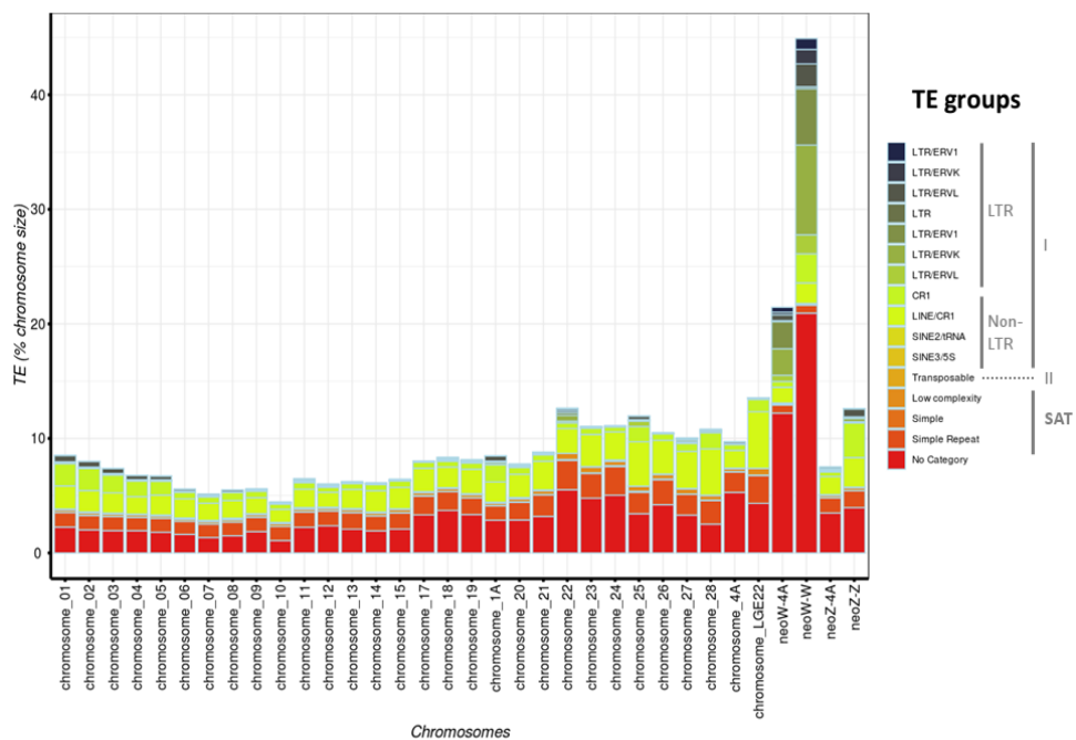
Figure S9. TE density for each chromosome and for each RepBase TE family. Class I TE elements were categorized following the two subclasses: LTR and non-LTR retrotransposons.
