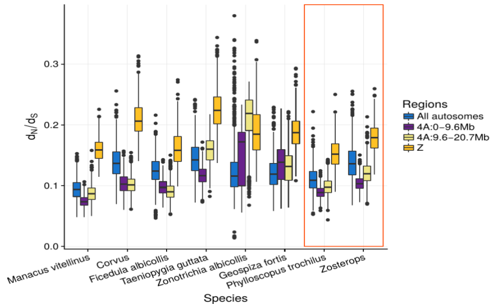
Figure 6. Variation in d_N/d_S ratios among chromosomal regions for the 11 investigated species. Estimates are performed at the genus level, i.e. on branches before the split of the two Corvus ( C. cornix and C. brachyrhynchos ) and the three Zosterops species ( Z. lateralis , Z. pallidus and Z. borbonicus ). The red box shows species with the translocated neoZ-4A region. For these species, the 4A:0-9.6 Mb region corresponds to the neoZ-4A and the Z corresponds to the neoZ-Z.
