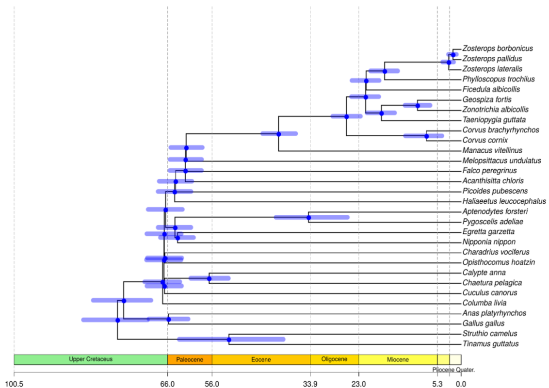
Figure S3. Molecular dating of the 30 birds species. Molecular dating estimates are based on the dataset 1 with CAT GTR substitution model, log-normal molecular rate model and calibration set 1 (Table S3).
