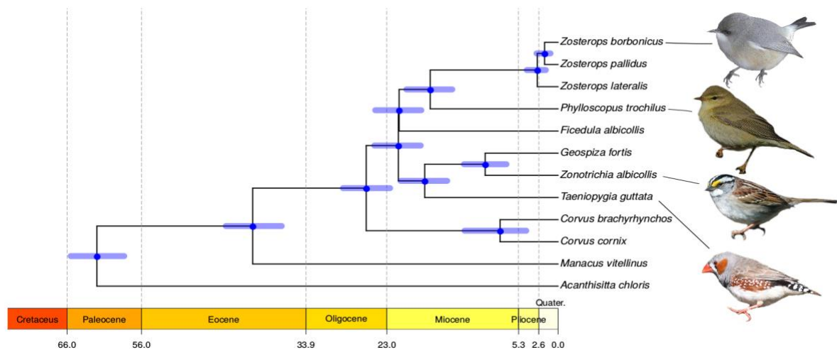
Figure 3. Molecular phylogeny and dating of the investigated passerine birds. Estimates of molecular dating are based on dataset 1 and calibration set 1 (Table S3). For greater clarity, the cladogram focuses on passerine birds only, but see Fig S3 for a cladogram of the inferred phylogeny for the whole set of investigated avian species.
