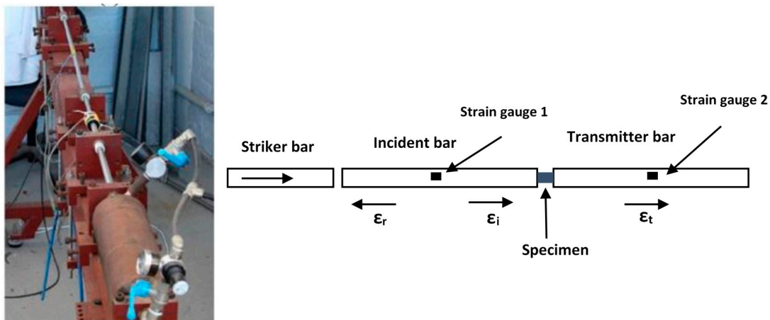
Figure 1. The SHPB compression test setup, reproduced from [29], with permission from Elsevier, 2019.
