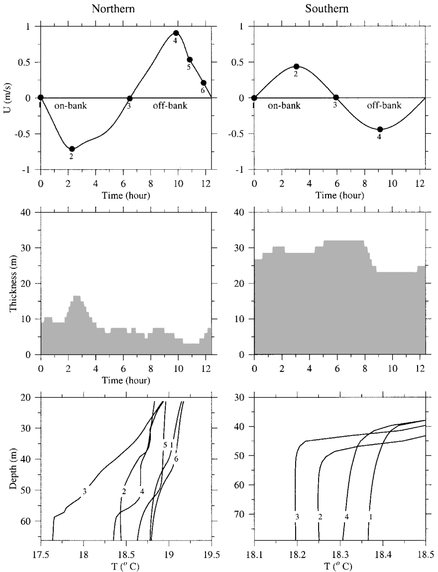
Figure 7. Time series of surface cross-bank current (top), height of the bottom mixed layer (middle), and vertical profile of temperature (bottom) over a tidal cycle at sites A and C on southern (right) and northern (left) flanks.
