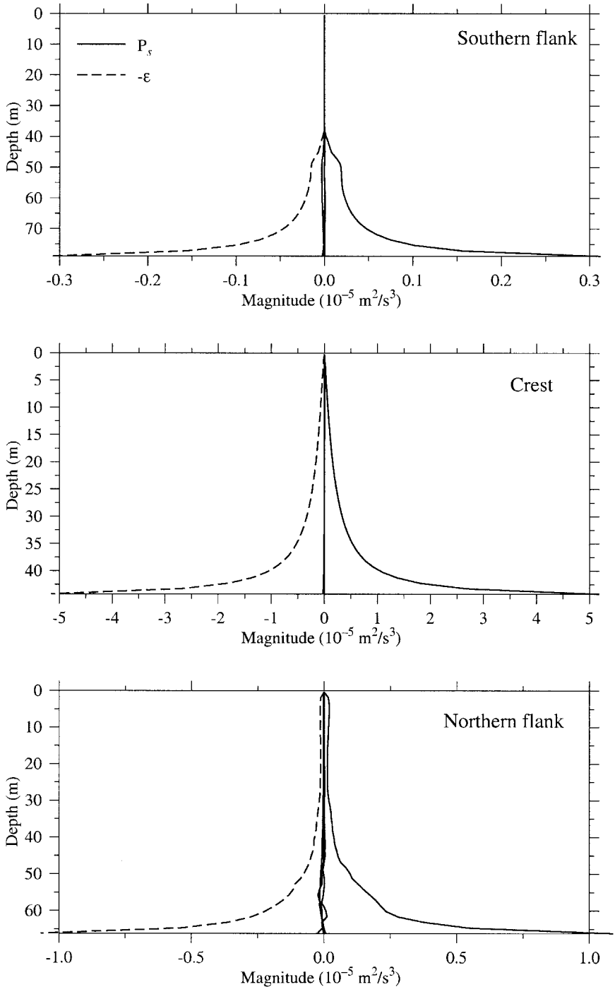
Figure 12. Vertical distribution of major terms in the turbulent kinetic energy equation at site A (southern flank), site B (crest), and site C (northern flank). All terms are averaged over a tidal cycle on the 15th model day.
