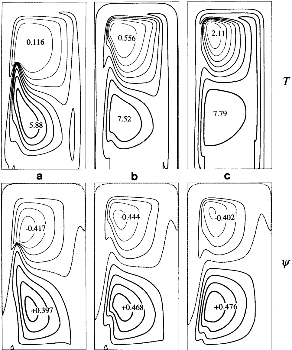
Figure 6. The transport streamfunction \psi (bottom) and surface temperature T (top) in three solutions of the toy model equations (3.5, 3.21) with \epsilon = 0.04 , \lambda = 1.0 , T_0 = 5.0 and \Delta = 0.2 . The solutions differ only in the value \xi_0 of (3.29) at which the temperature changes most rapidly: (a) \xi_0 = 0.0 ; (b) \xi_0 = -0.2 ; (c) \xi_0 = -0.35 . The temperature transition thus occurs at a progressively more subpolar value of (3.29) in the sequence (a-c).
