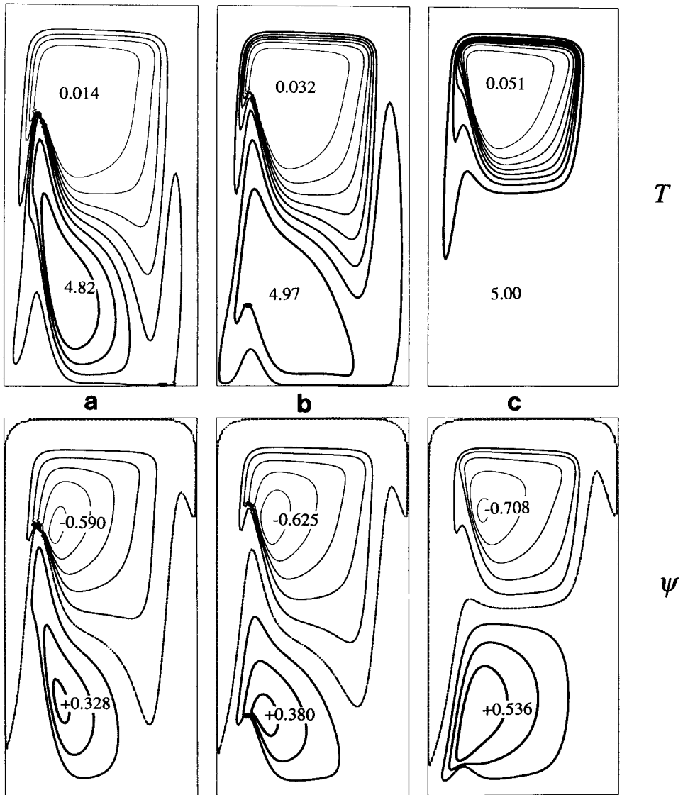
Figure 3. The streamfunction \psi (bottom) and temperature T (top) in three solutions of the toy model equation (2.20) with depth-invariant temperature given by (2.24). In all three solutions \epsilon = 0.02 , T_0 = 5.0 and \Delta = 0.2 . The solutions differ only in the location of the temperature transition line: (a) \psi_0 = 0.0 (b) \psi_0 = -0.12 (c) \psi_0 = -0.25 . The transition thus occurs on a progressively more subpolar streamline in the sequence (a-c).
