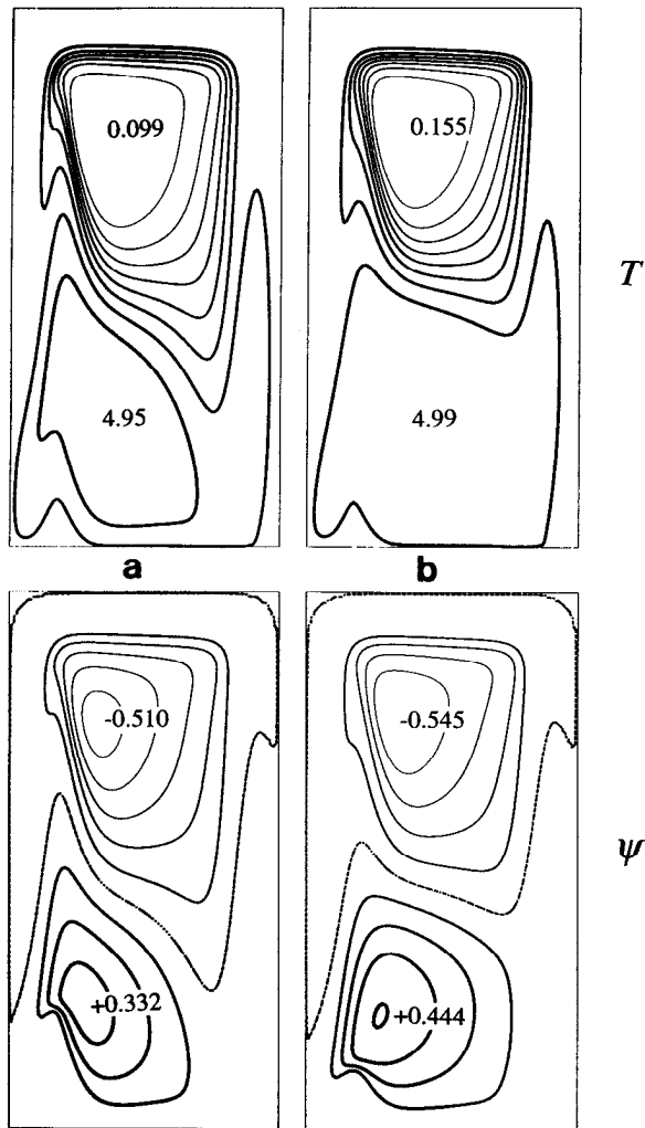
Figure 7. The transport streamfunction \psi (bottom) and temperature (top) in two solutions of the toy model equations (2.20, 2.24) with depth-independent temperature, \lambda = 0.0 . In both solutions, \epsilon = 0.04 , T_0 = 5.0 and \Delta = 0.2 . The two solutions differ only in the value \psi_0 of the streamfunction where the temperature changes most rapidly: (a) \psi_0 = -0.12 ; and (b) \psi_0 = -0.2 . These solutions differ from those in Figure 3 in their higher friction. They differ from those in Figure 6 in the value of the stratification parameter \lambda .
