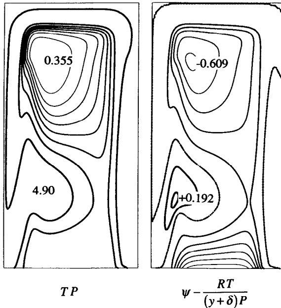
Figure 5. The depth-averaged temperature (left) and the quantity (3.29) in the solution presented in Figure 6b. According to the toy-model temperature equation (3.20), the Jacobian of these two quantities must vanish.
