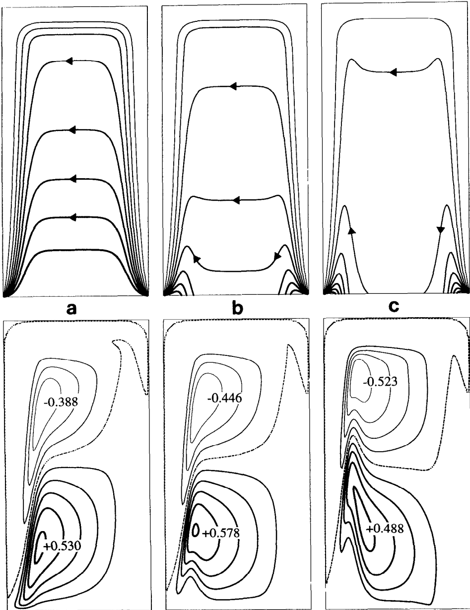
Figure 2. The transport streamfunction \psi (bottom) in three solutions of the toy model equation (2.20) with depth-invariant temperature given by the linear relation (2.23). All three solutions have \epsilon = 0.015 , and differ only in the value of the coefficient T_0 in (2.23): (a) T_0 = 0.0 (homogeneous fluid); (b) T_0 = 2.0 ; (c) T_0 = 5.0 . Thus, the sequence (a–c) corresponds to increasing temperature contrast within the fluid. Darker contours correspond to larger values of \psi , and extremal values are shown. The top panels show the corresponding ‘streamfunction’ (2.21) for the ‘flow’ ‘advecting’ \psi in (2.20), with ‘flow’ direction indicated by the arrows.
