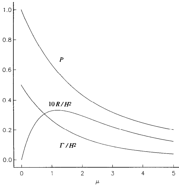
Figure 4. The three functions P(H) , R(H) and \Gamma(H) that appear in the toy model, shown as functions of the parameter \mu = \lambda H , where H is the ocean depth and \lambda^{-1} is the decay-depth for temperature.
