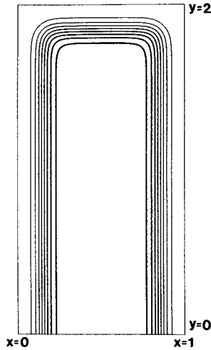
Figure 1. The ocean basin topography used for all solutions. The ocean depth varies between 0 and 1, and vanishes smoothly at the western, northern, and eastern boundaries. The southern, equatorial boundary is open.
