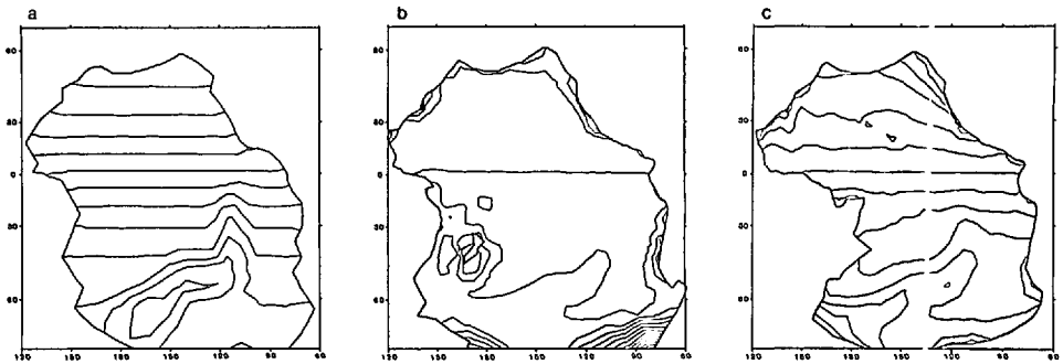
Figure 5. Contours of constant f/H in model Pacific basins for (a) 2500 m-high model Pacific Rise in an otherwise constant depth ocean of 5000 m depth ( CI = 5.2 \times 10^{-9} \text{ m}^{-1} \text{ s}^{-1} ), (b) Rand/SIO topography smoothed to the high resolution of the eigenmodel ( CI = 2.9 \times 10^{-8} \text{ m}^{-1} \text{ s}^{-1} ), and (c) Rand/SIO topography smoothed as in (b) but reduced-Pacific geometry such that the near-coastal and Fiji/New Zealand regions of steep and poorly resolved f/H are excised from the domain ( CI = 7.3 \times 10^{-9} \text{ m}^{-1} \text{ s}^{-1} ).
