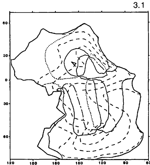
Figure 10. Reduced-Pacific geometry with Rand/SIO topography and high resolution. Plotted as in Figure 2, but for the fundamental planetary-topographic mode of the Pacific with period = 3.1 days.
