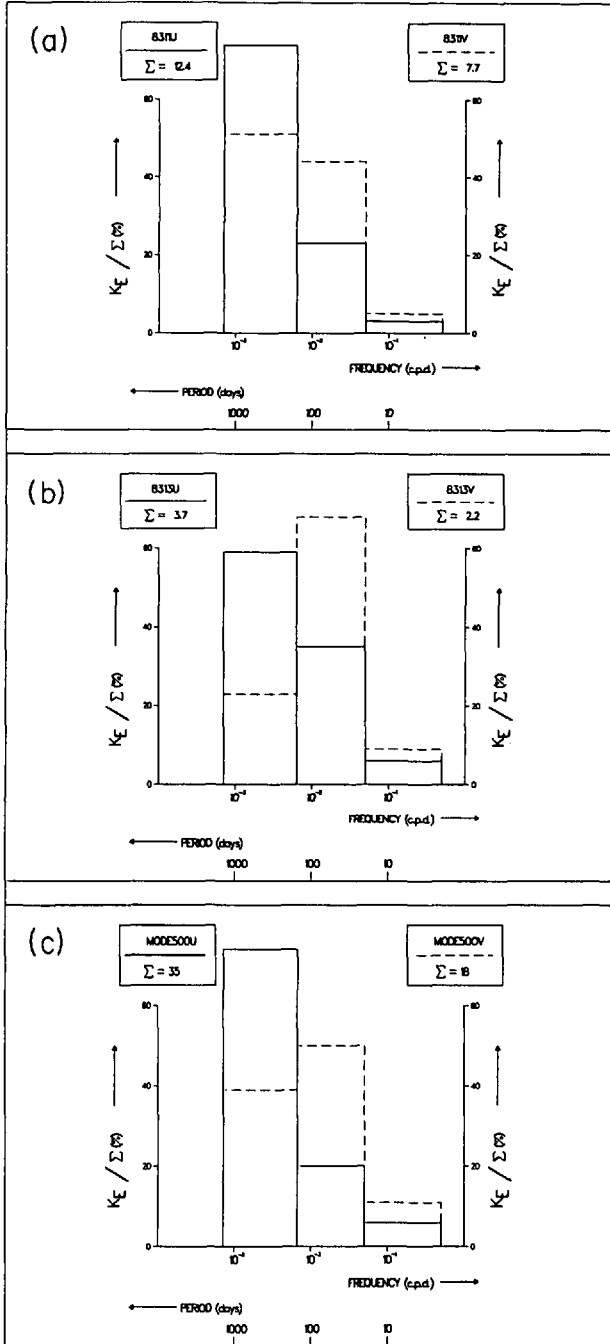
Figure 12. Normalized frequency distributions for the zonal and meridional contributions to K_E : (a) 470 m, 8311; (b) 1070 m, 8313; (c) at 500 m depth (nominal) from the central MODE site (28N, 70W).
