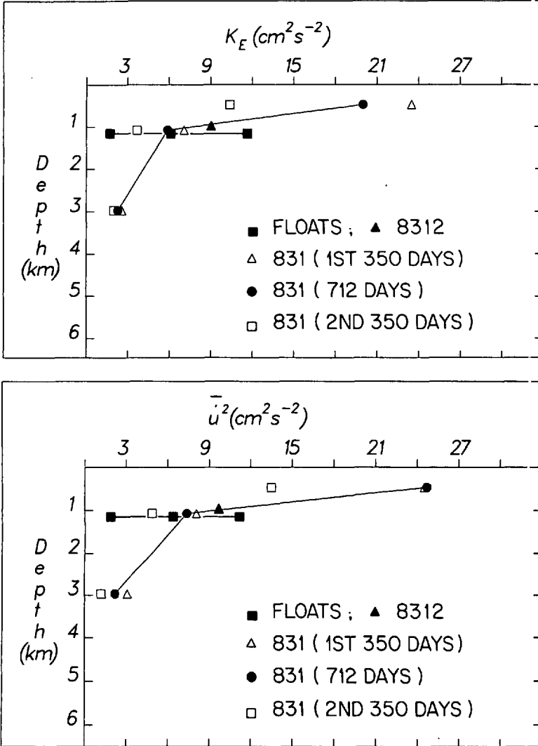
Figure 9. Vertical distribution of the eddy field time-averages, along with the float cluster data near 1100 m depth: (a) eddy kinetic energy K_E ; (b) zonal variance, \bar{u}^2 ; (c) \bar{v}^2 , meridional variance. Solid dots connected by a line are for 2-year averages of the moored instrument observations, open triangles and squares for averages respectively based only on the first or second year's data. A solid triangle denotes 8312 (329-day record, first year) and solid squares connected by a line indicate respectively the minimum, mean, and maximum values for the float cluster deployed near mooring 831 (32N, 24W, Fig. 1).
