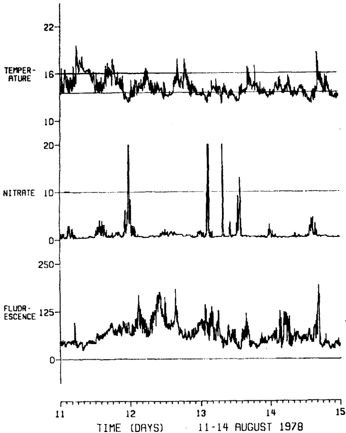
Figure 6. Time series of temperature, nitrate concentration, and fluorescence at 11 m depth 11-14 August, 1978. The line at 13.5° is drawn to illustrate that nitrate concentration rises above the background level when temperature dips below 13.5°.
