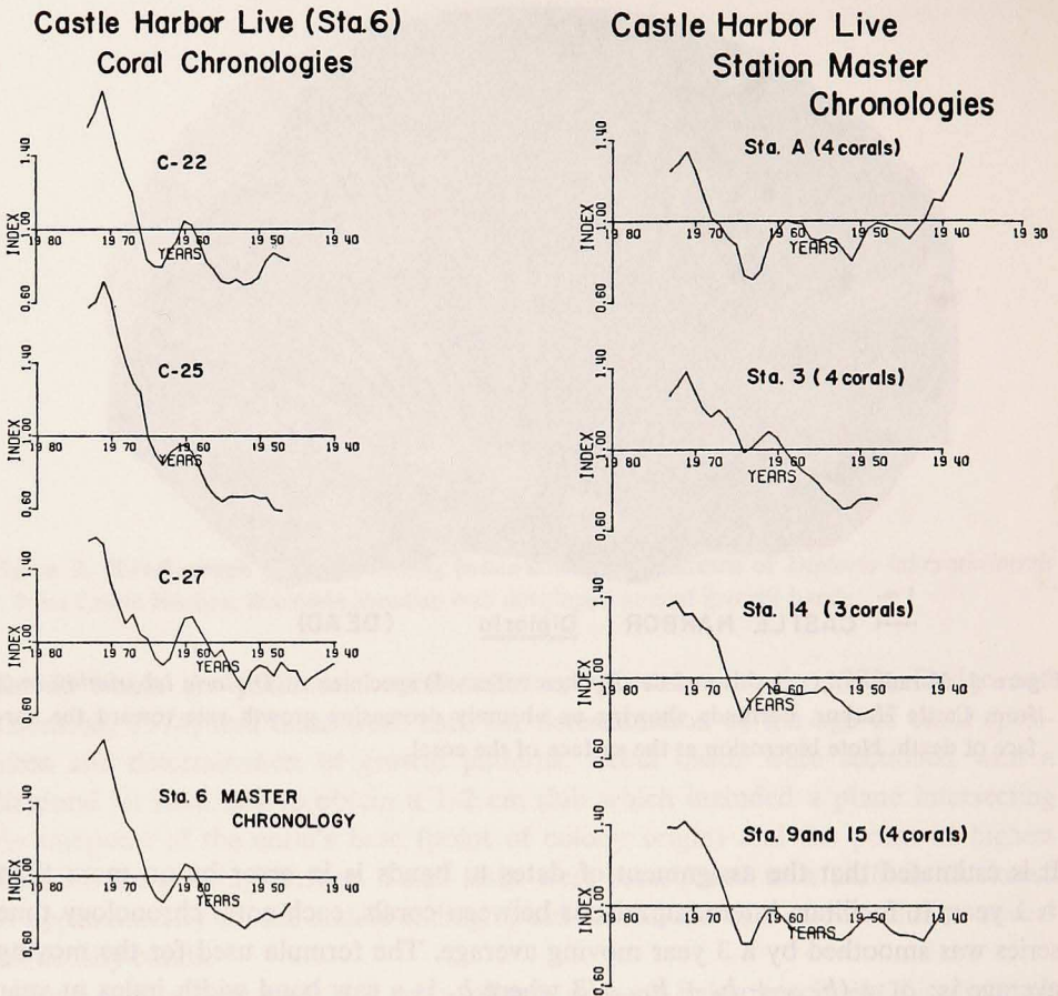
Figure 5. Band width chronologies (time series of band widths, each plotted as index value or the percentage of the average coral growth rate) for typical coral colonies at Station 6 in Castle Harbor. The station summary or chronology is also shown. This is the average by year of coral chronologies at the station.
