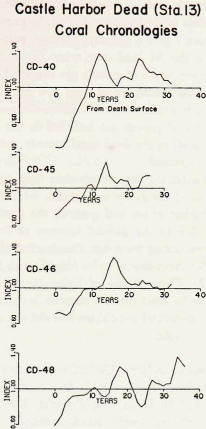
Figure 7. Chronologies of several representative dead corals from Station 13 in Castle Harbor. Yearly growth rates (normalized to the coral mean) are plotted from left to right beginning at the band approximately coincident with death.
