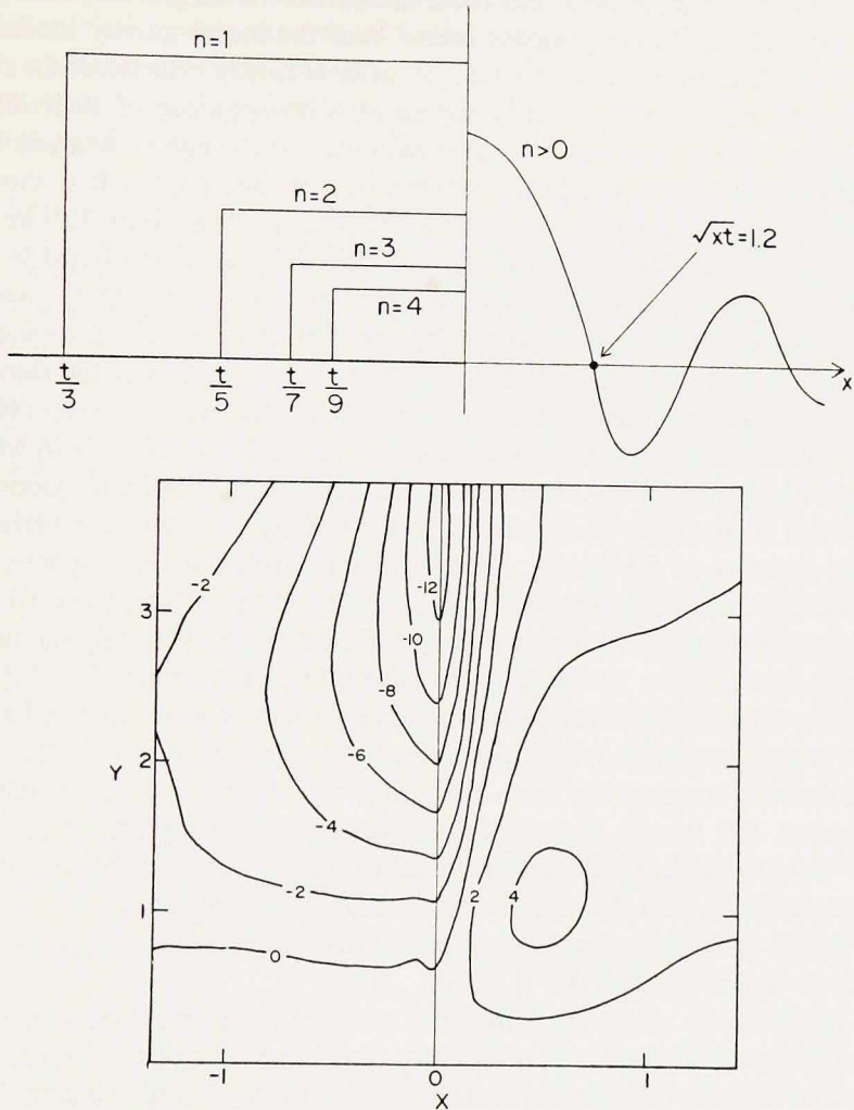
Figure 10. Unbounded baroclinic response to a step function southerly wind (a). The longitudinal dependence of the low n modes. (b) The layer depth h at t = 9 for the case G = H(x) , F = Q = 0 .
