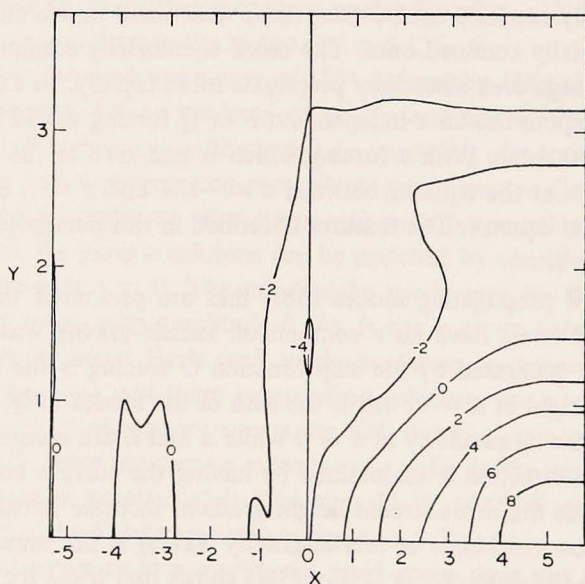
Figure 9. Unbounded baroclinic response to a step function westerly wind. (a) The longitudinal dependence of the low n modes. (b) The layer depth h at t = 5 for the case F = H(x) , G = Q = 0 .
