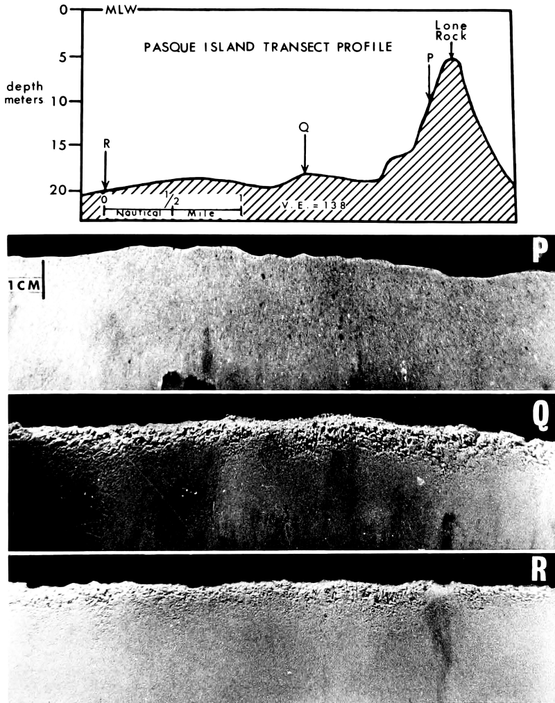
Figure 6. Diagrammatic profile of the Pasque Island transect and in situ surface sediment photographs taken at Sts. P, Q, and R. Sts. Q and R, which are populated by deposit-feeding bivalves, show a granular burrowed surface.
