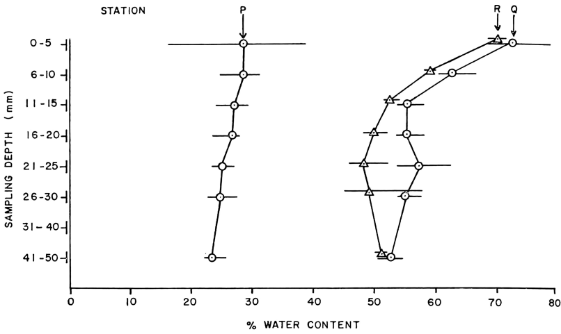
Figure 12. Water content of cores from the Pasque Island transect. Sts. Q and R—extensively burrowed by deposit feeders—have a high surface-water content. St. P, dominated by suspension feeders, is uniformly low in water content. The mean of four cores is plotted with the range of values (horizontal bar).
