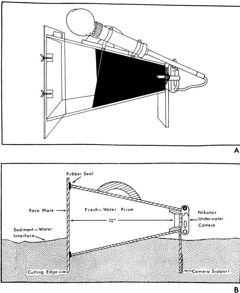
Figure 3. Sediment-water interface camera. (A) Lateral view showing the plexiglass pyramid attached to a Nikonos underwater camera, the apical part of the fresh-water prism, painted black to decrease backscatter of light, and Nikonos flash unit used to illuminate the sediment water interface profile. (B) Cross-section showing the camera placed in position (by a diver) to photograph the sediment surface in profile.
