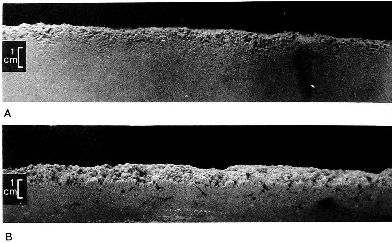
Figure 8. Development of a granular surface by the near-surface burrowing activities of Numa proxima . In situ profile of the granular surface at (A) St. R and (B) in an aquarium.
