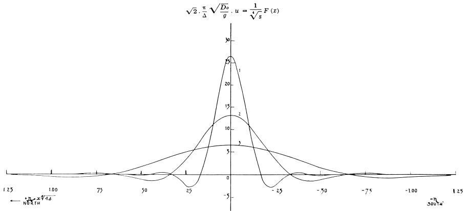
Figure 8. Successive velocity profile, computed for s_1 = 0.055 \cdot 10^{-4} , s_2 = 16s_1 , s_3 = 16s_2 , and plotted against the non-dimensional transversal coordinate \eta . To obtain actual velocities from the non-dimensional ordinates plotted in the figure, the latter must be multiplied with the constant factor \frac{\Delta}{\pi} \sqrt{\frac{g}{D_0}} \cdot \frac{1}{\sqrt{2}} .
