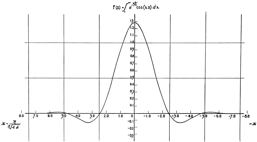
Figure 7. Non-dimensional representation of velocity distribution as a function of \frac{\eta}{\sqrt{4s}} taking into consideration the Coriolis' force acting upon the transversal velocity components. The ordinate is 1.2818 u/u_o , where u_o is the simultaneous velocity in the center of the current.
