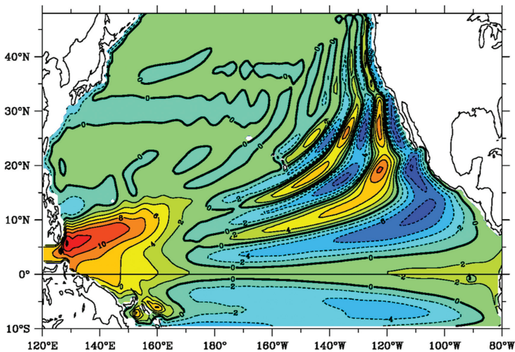
Figure 6. An example of Rossby wave propagation generated by equatorial wind variations shows the response to Kelvin waves in the form of Rossby waves propagating westward from the American continental coasts. The waves refract toward the poles due to changes in phase speed with latitude. Image provided courtesy of B Qiu.
