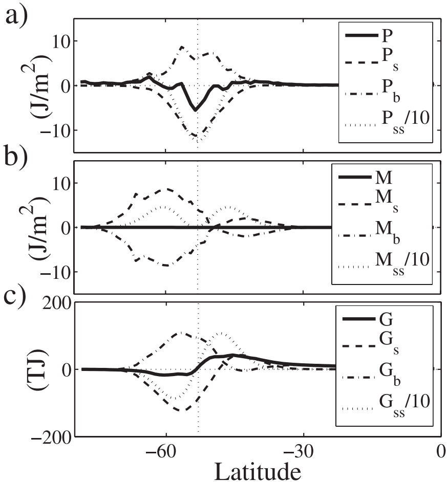
Figure 7. (a) Zonally-averaged pressure work P and (b) divergence contribution to the potential energy equation M , and (c) zonally integrated meridional flux of energy G . Contributions of surface layer (dashed) and barotropic interior (dash-dotted) add up to total (solid). Dotted lines denote the P_{s,s} , M_{s,s} and G_{s,s} terms (attenuated by a factor of 10) which would reflect P_s , M_s and G_s if divergences of the Ekman transport were the only factors able to deform the surface. See text for explanation.
