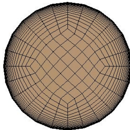
Fig. 2 Fluid Domain Mesh y^+ \approx 5 (viscous sublayer)
