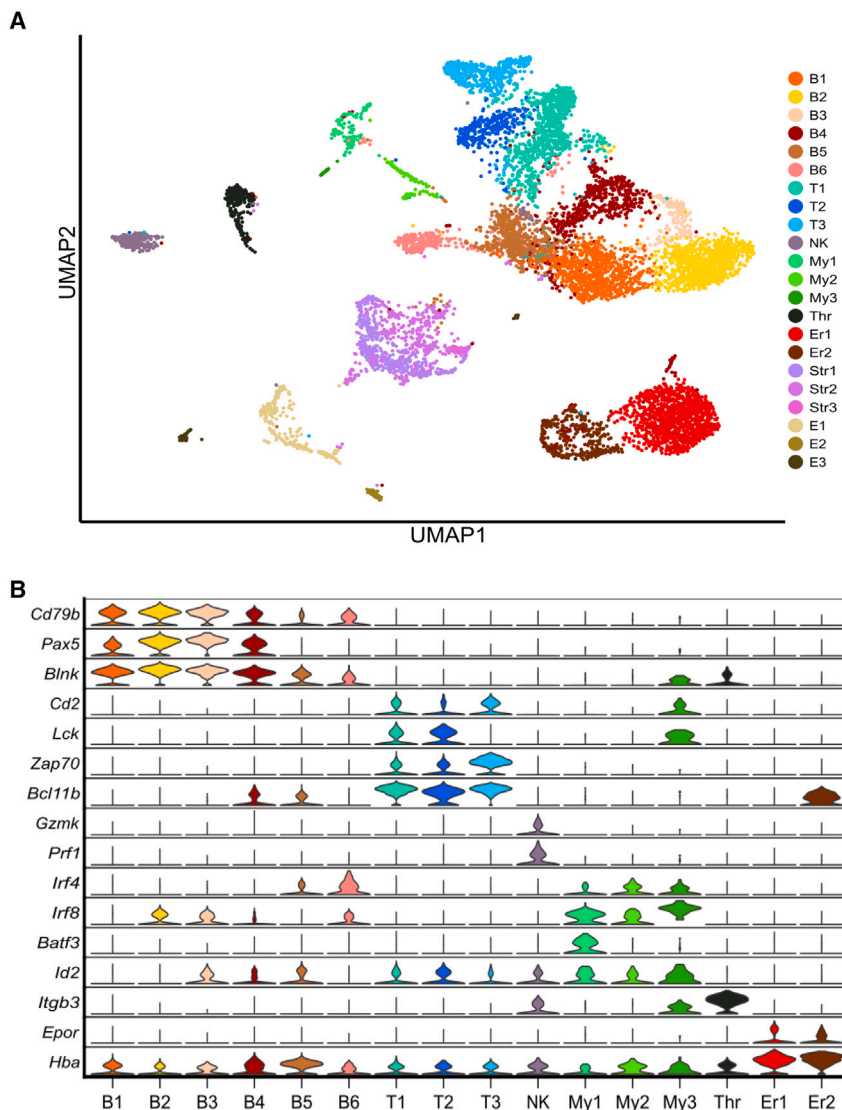
Figure 1. Single-cell transcriptome of the nurse shark spleen post-immunization
