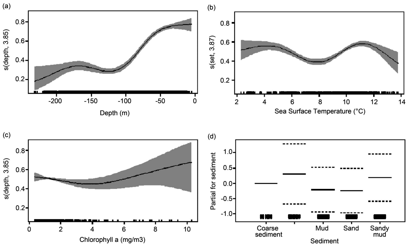
Fig. 3. Generalised additive model (GAM) plots showing the relationship between minke whale sightings and explanatory variables: a) depth (m); b) sea surface temperature (°C); c) chlorophyll concentration (mg/m 3 ); d) sediment type. The y-axis represents the probability of a minke whale sighting, assuming other variables are at their average value. Black marks on the x-axis represent the total distribution of data. Black line represents the best-fitted trend line. Grey area represents 95% confidence intervals of the trend line. N = 4,564 .
